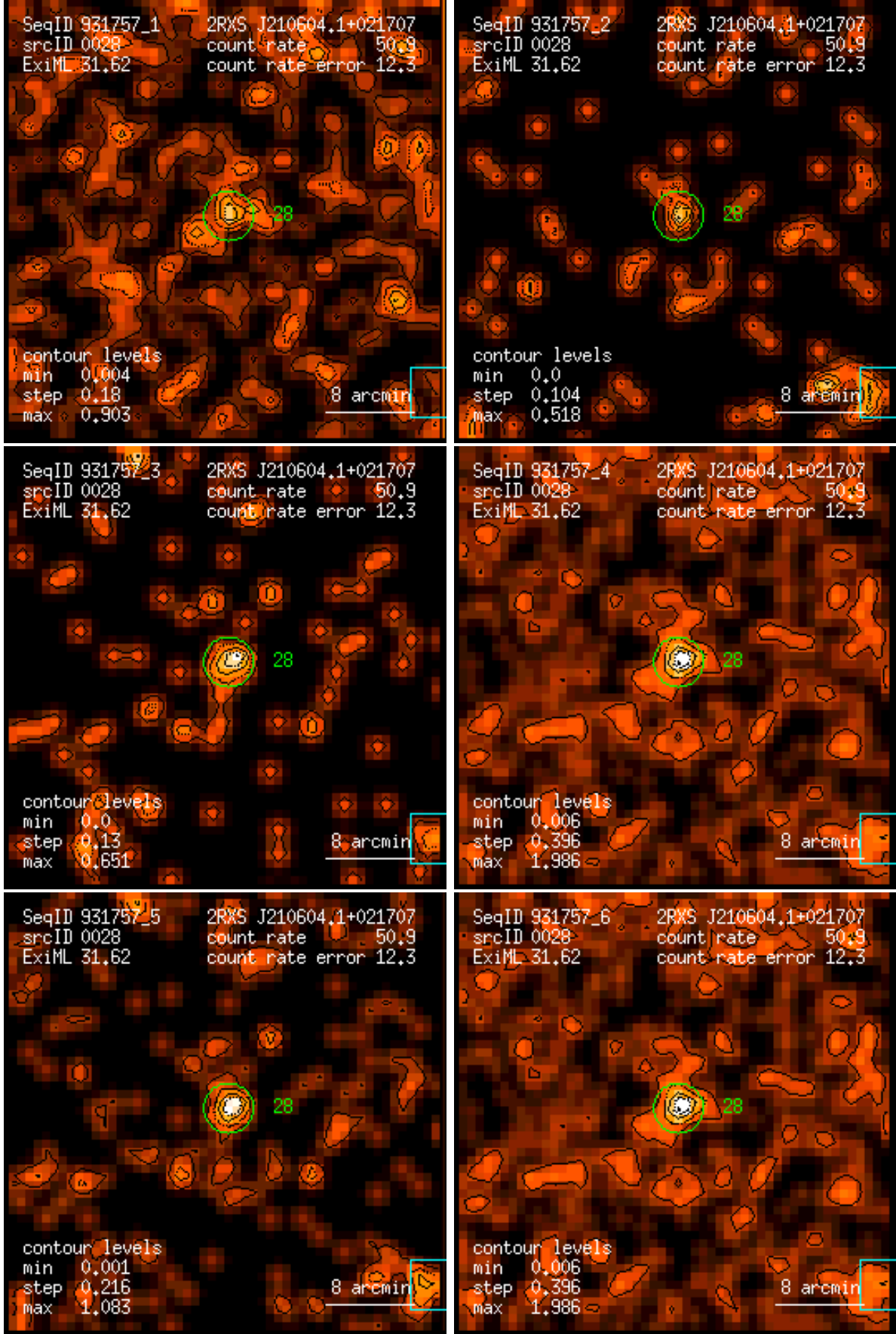
Figure 28: RASS 931757: detection 0028: band rate images, Gaussian filter: (1) PSPC channels 11 – 41, (2) 52 – 90, (3) 91 – 201, (4) 11 – 235, (5) 52 – 201, (6) 11 – 201. Broad band rates in counts/ks. Band rate contour levels in counts/ks/arcmin 2 .
