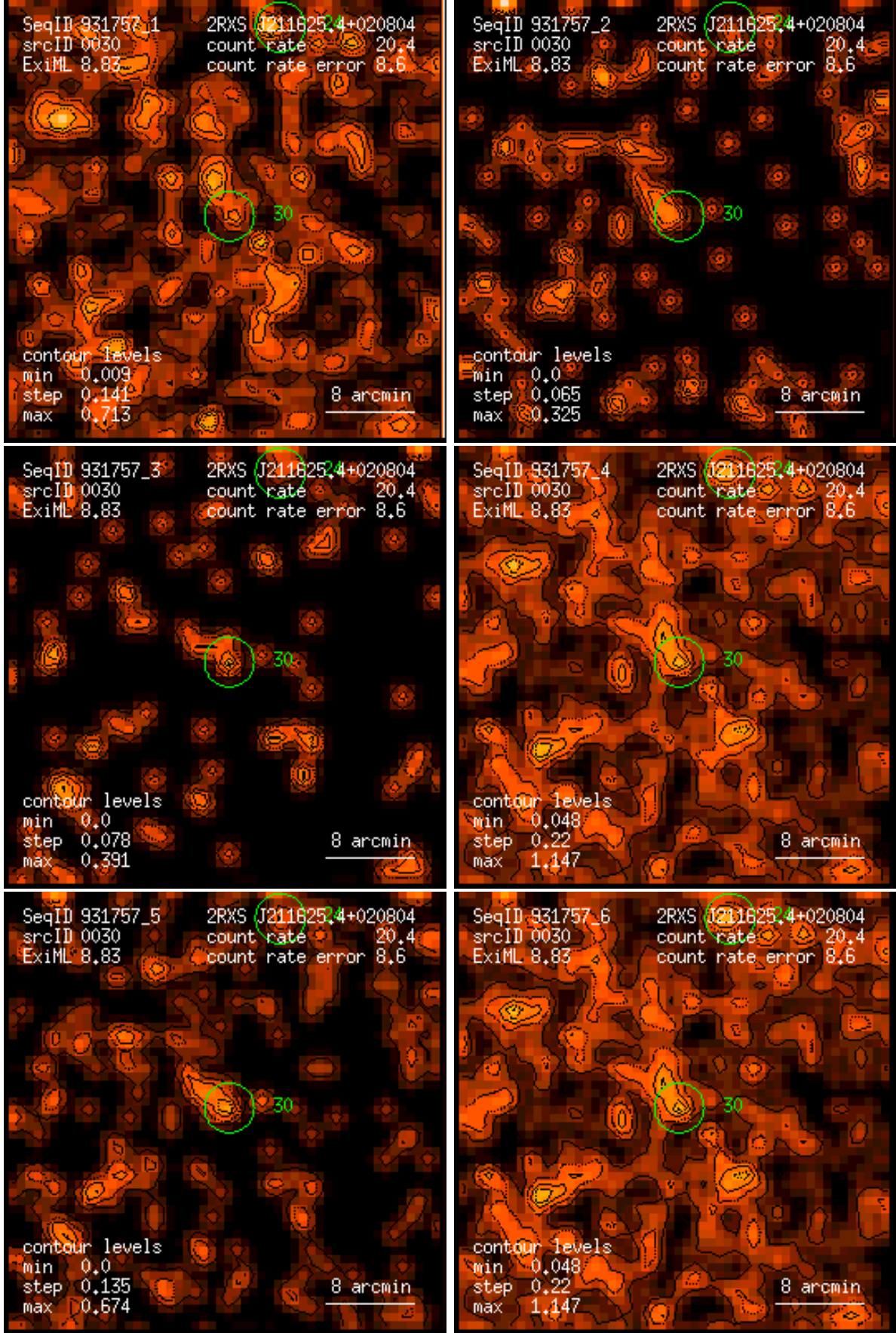
Figure 30: RASS 931757: detection 0030: band rate images, Gaussian filter: (1) PSPC channels 11 – 41, (2) 52 – 90, (3) 91 – 201, (4) 11 – 235, (5) 52 – 201, (6) 11 – 201. Broad band rates in counts/ks. Band rate contour levels in counts/ks/arcmin 2 .
