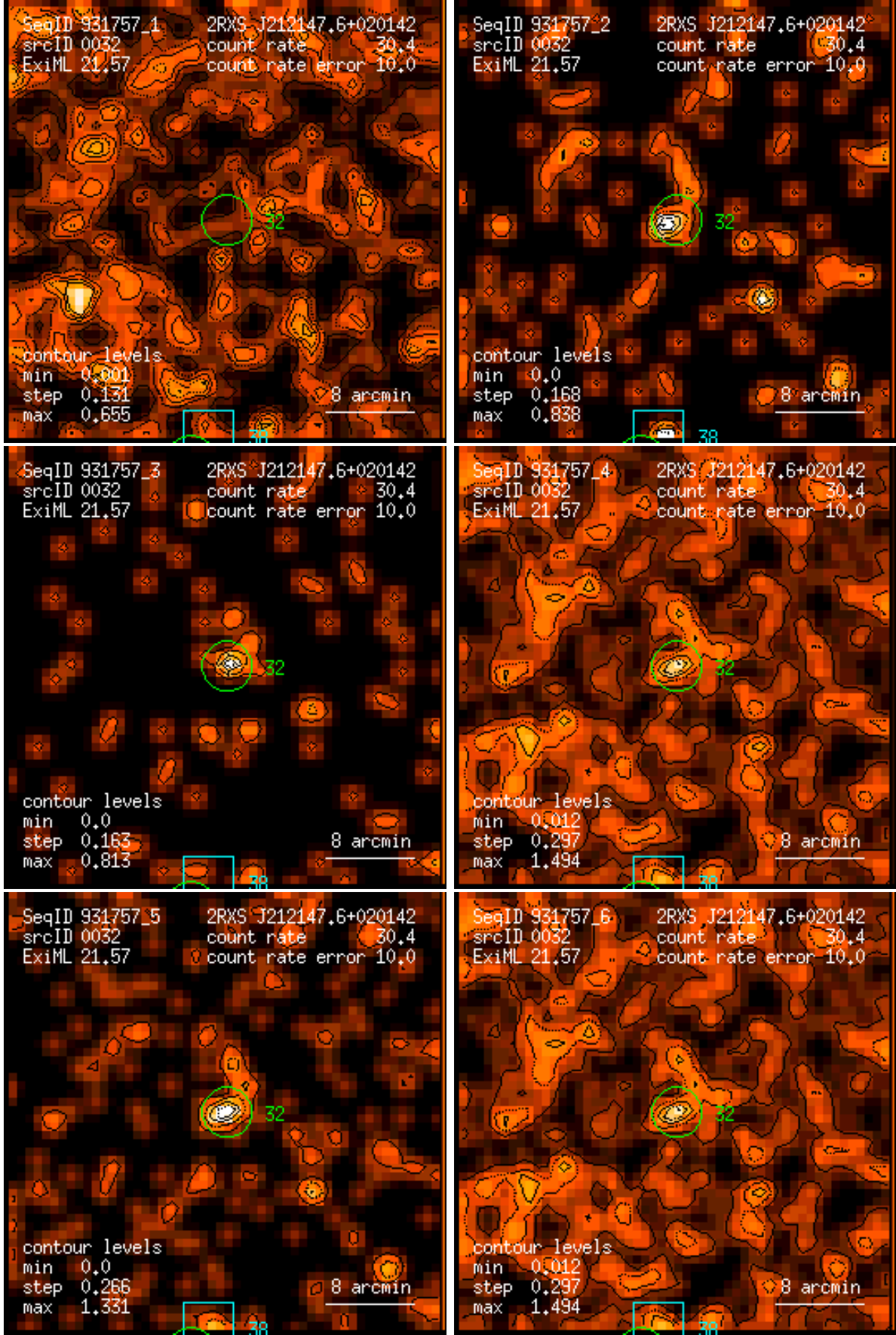
Figure 32: RASS 931757: detection 0032: band rate images, Gaussian filter: (1) PSPC channels 11 – 41, (2) 52 – 90, (3) 91 – 201, (4) 11 – 235, (5) 52 – 201, (6) 11 – 201. Broad band rates in counts/ks. Band rate contour levels in counts/ks/arcmin 2 .
