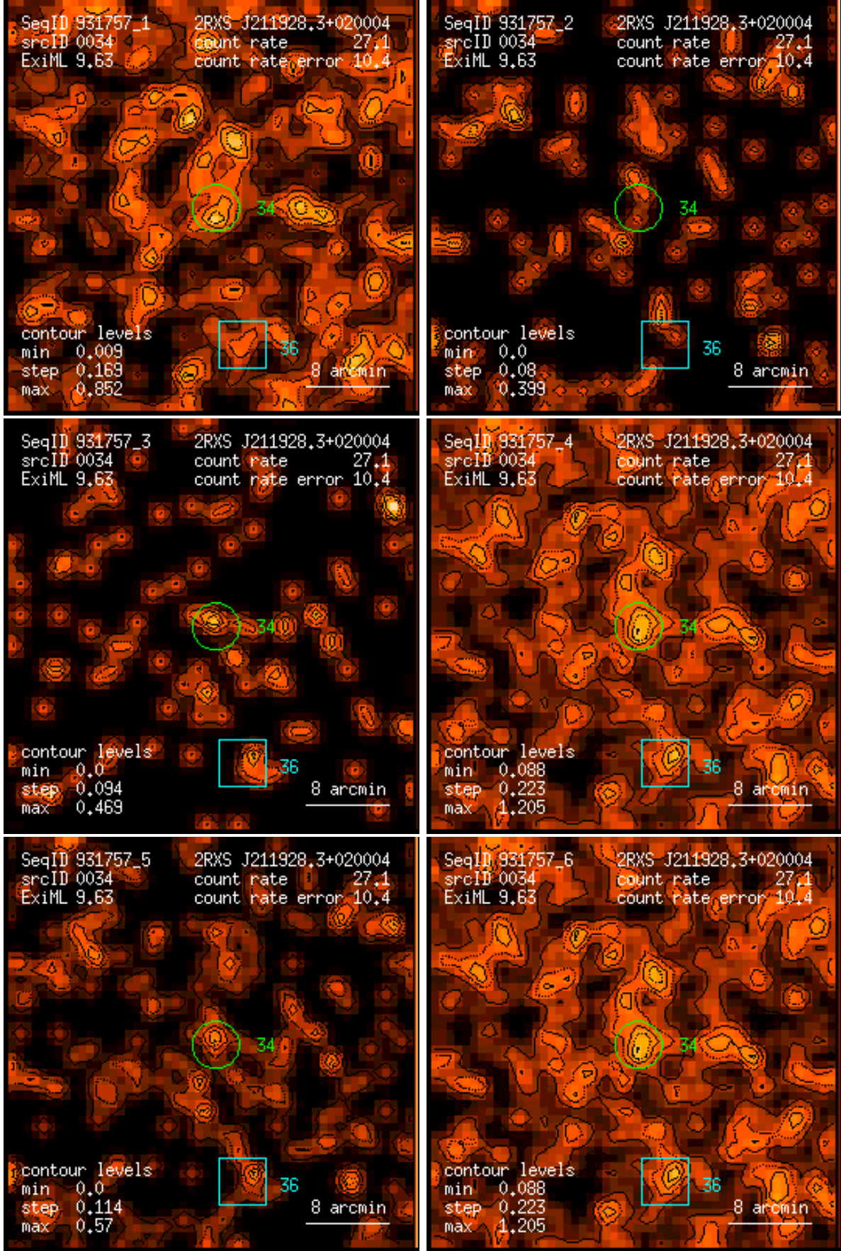
Figure 34: RASS 931757: detection 0034: band rate images, Gaussian filter: (1) PSPC channels 11 – 41, (2) 52 – 90, (3) 91 – 201, (4) 11 – 235, (5) 52 – 201, (6) 11 – 201. Broad band rates in counts/ks. Band rate contour levels in counts/ks/arcmin 2 .
