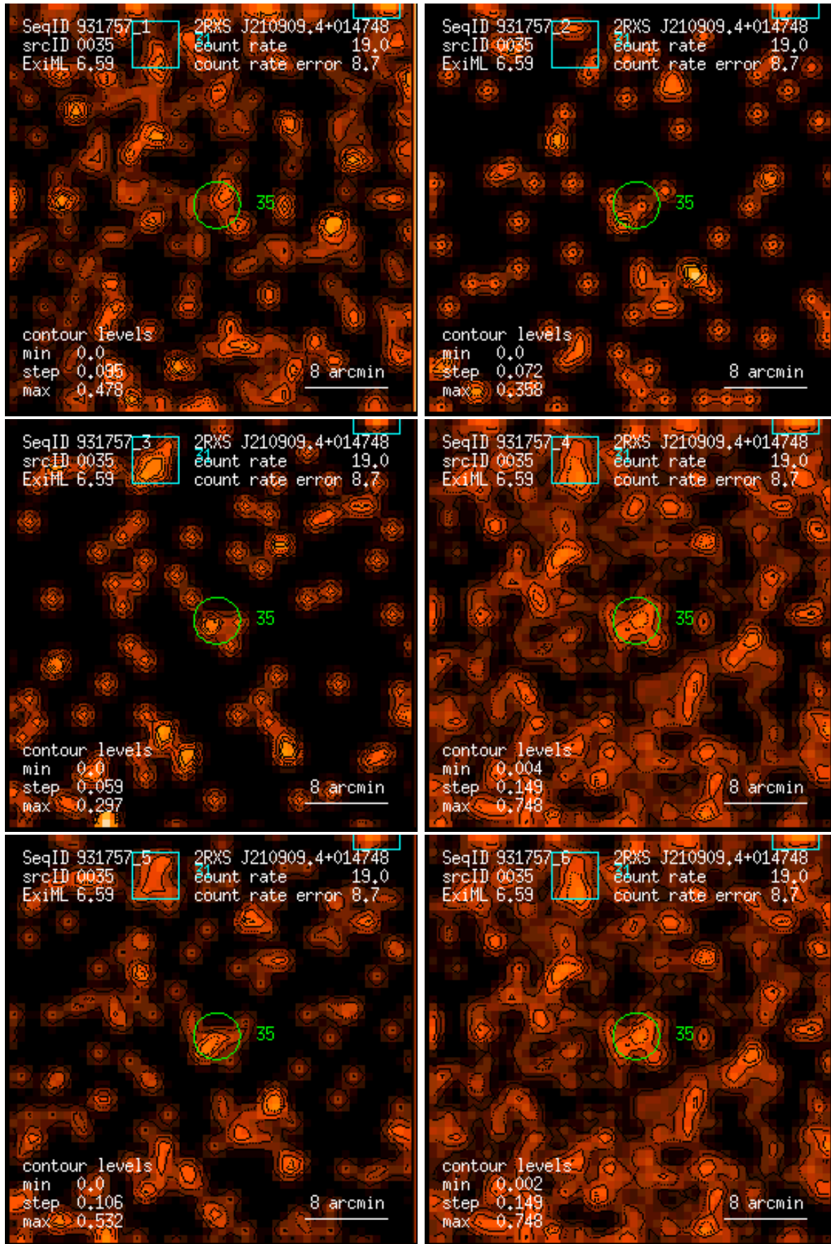
Figure 35: RASS 931757: detection 0035: band rate images, Gaussian filter: (1) PSPC channels 11 – 41, (2) 52 – 90, (3) 91 – 201, (4) 11 – 235, (5) 52 – 201, (6) 11 – 201. Broad band rates in counts/ks. Band rate contour levels in counts/ks/arcmin 2 .
