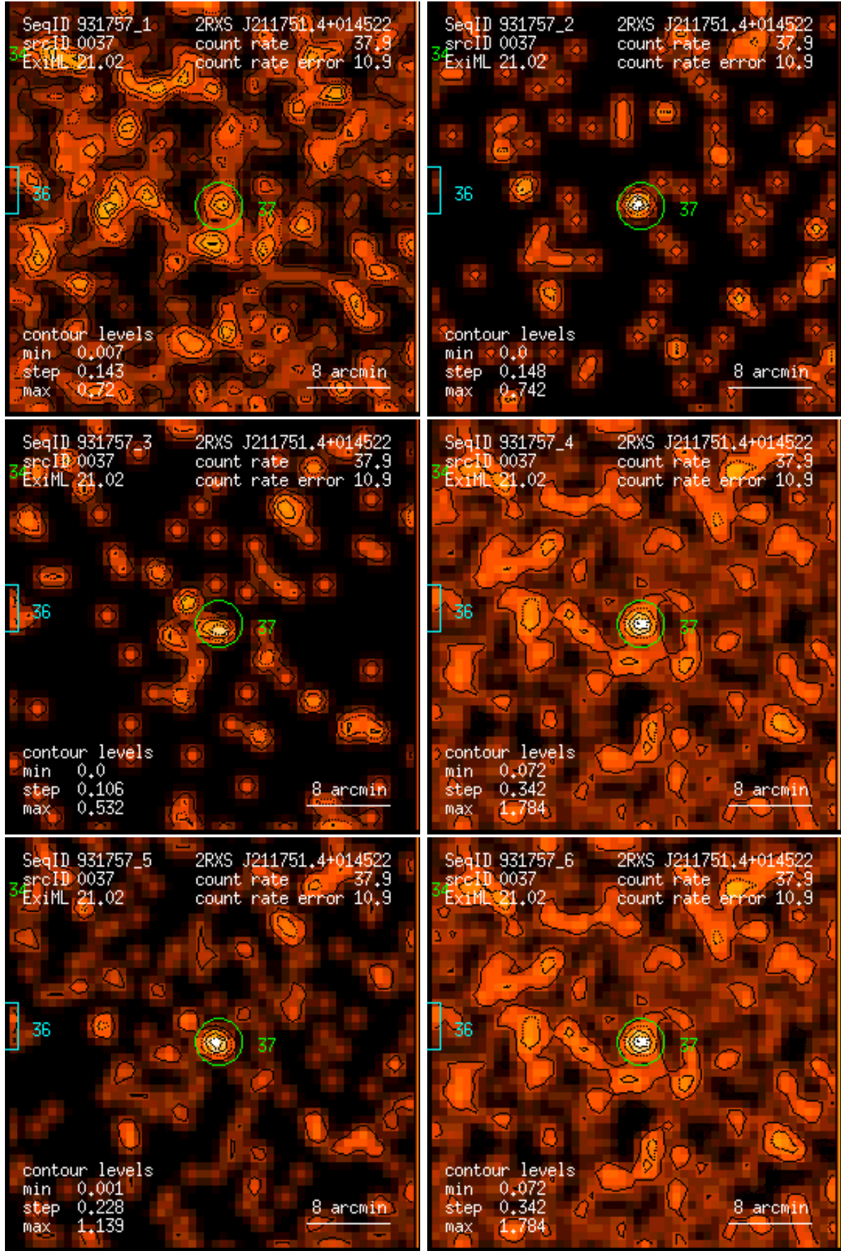
Figure 37: RASS 931757: detection 0037: band rate images, Gaussian filter: (1) PSPC channels 11 – 41, (2) 52 – 90, (3) 91 – 201, (4) 11 – 235, (5) 52 – 201, (6) 11 – 201. Broad band rates in counts/ks. Band rate contour levels in counts/ks/arcmin 2 .
