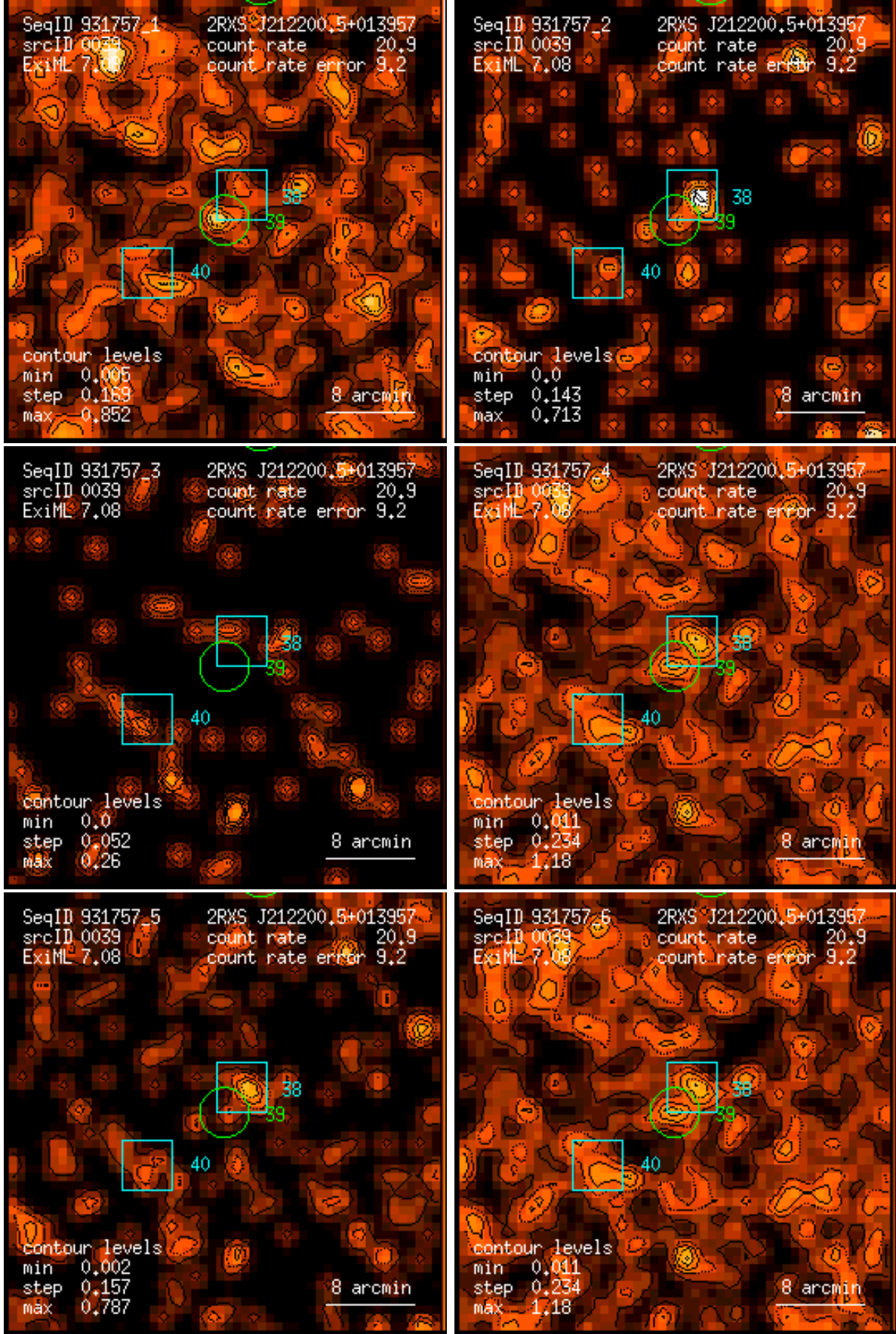
Figure 39: RASS 931757: detection 0039: band rate images, Gaussian filter: (1) PSPC channels 11 – 41, (2) 52 – 90, (3) 91 – 201, (4) 11 – 235, (5) 52 – 201, (6) 11 – 201. Broad band rates in counts/ks. Band rate contour levels in counts/ks/arcmin 2 .
