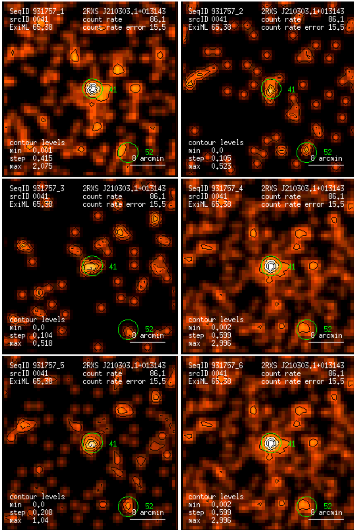
Figure 41: RASS 931757: detection 0041: band rate images, Gaussian filter: (1) PSPC channels 11 – 41, (2) 52 – 90, (3) 91 – 201, (4) 11 – 235, (5) 52 – 201, (6) 11 – 201. Broad band rates in counts/ks. Band rate contour levels in counts/ks/arcmin 2 .
