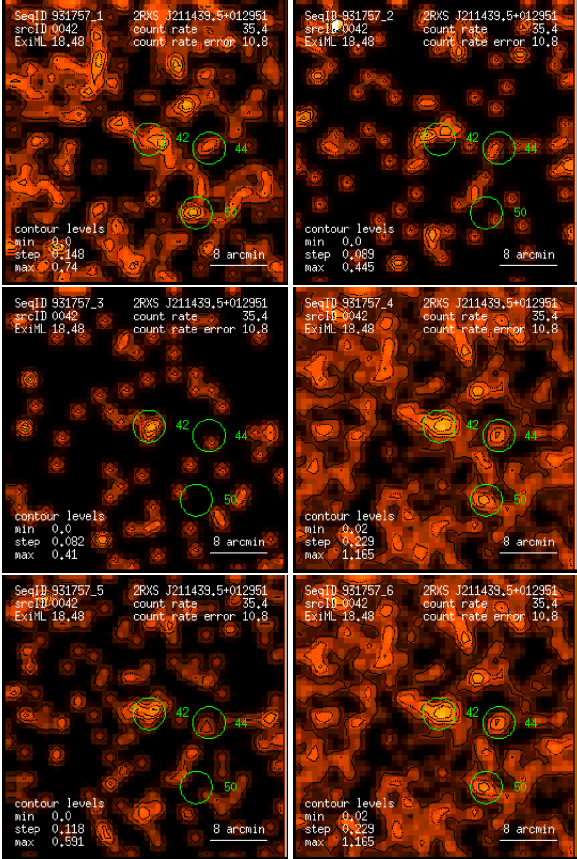
Figure 42: RASS 931757: detection 0042: band rate images, Gaussian filter: (1) PSPC channels 11 – 41, (2) 52 – 90, (3) 91 – 201, (4) 11 – 235, (5) 52 – 201, (6) 11 – 201. Broad band rates in counts/ks. Band rate contour levels in counts/ks/arcmin 2 .
