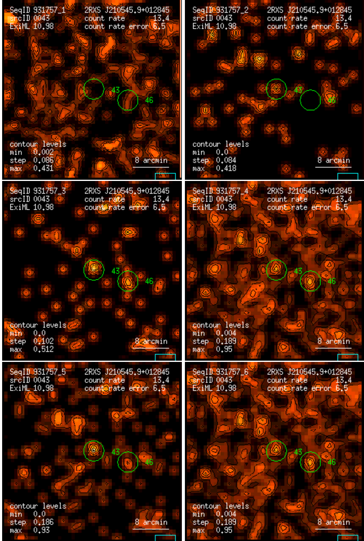
Figure 43: RASS 931757: detection 0043: band rate images, Gaussian filter: (1) PSPC channels 11 – 41, (2) 52 – 90, (3) 91 – 201, (4) 11 – 235, (5) 52 – 201, (6) 11 – 201. Broad band rates in counts/ks. Band rate contour levels in counts/ks/arcmin 2 .
