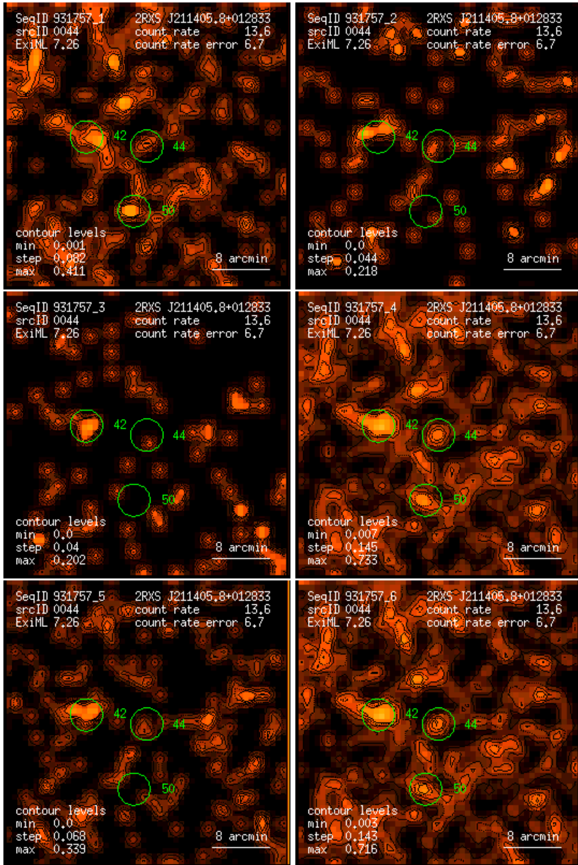
Figure 44: RASS 931757: detection 0044: band rate images, Gaussian filter: (1) PSPC channels 11 – 41, (2) 52 – 90, (3) 91 – 201, (4) 11 – 235, (5) 52 – 201, (6) 11 – 201. Broad band rates in counts/ks. Band rate contour levels in counts/ks/arcmin 2 .
