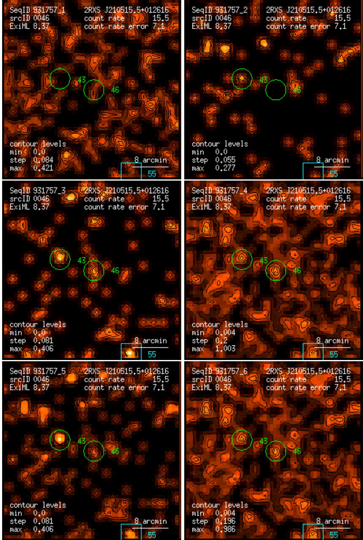
Figure 46: RASS 931757: detection 0046: band rate images, Gaussian filter: (1) PSPC channels 11 – 41, (2) 52 – 90, (3) 91 – 201, (4) 11 – 235, (5) 52 – 201, (6) 11 – 201. Broad band rates in counts/ks. Band rate contour levels in counts/ks/arcmin 2 .
