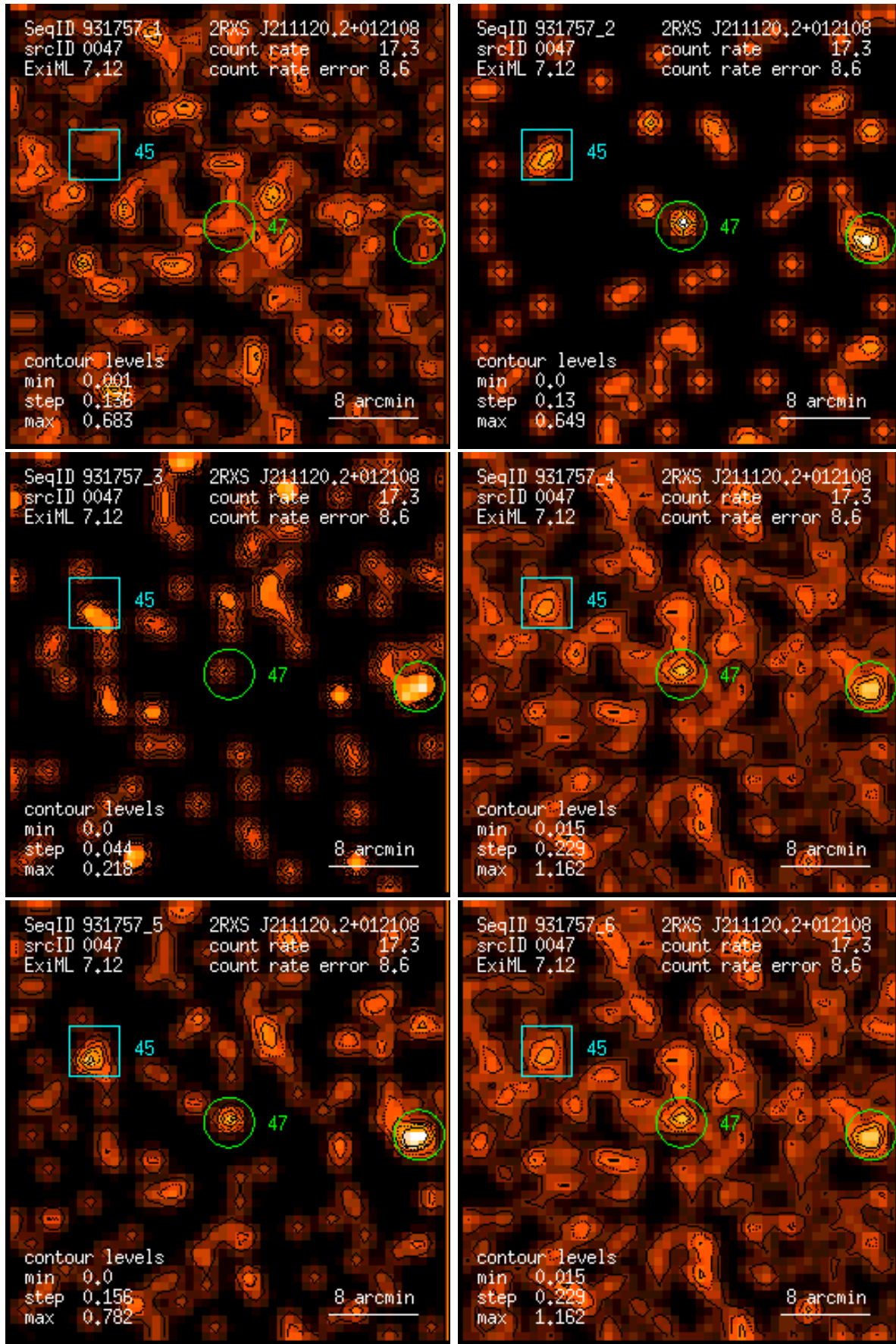
Figure 47: RASS 931757: detection 0047: band rate images, Gaussian filter: (1) PSPC channels 11 – 41, (2) 52 – 90, (3) 91 – 201, (4) 11 – 235, (5) 52 – 201, (6) 11 – 201. Broad band rates in counts/ks. Band rate contour levels in counts/ks/arcmin 2 .
