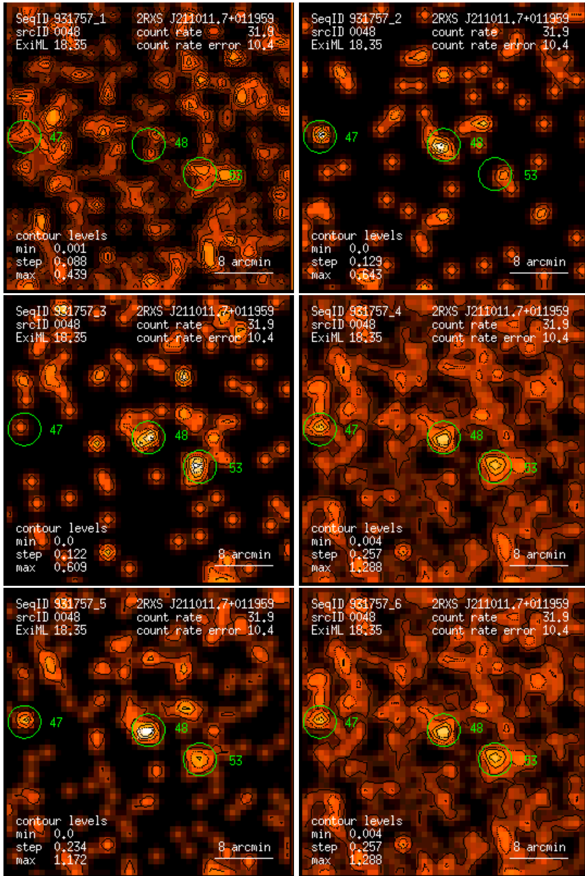
Figure 48: RASS 931757: detection 0048: band rate images, Gaussian filter: (1) PSPC channels 11 – 41, (2) 52 – 90, (3) 91 – 201, (4) 11 – 235, (5) 52 – 201, (6) 11 – 201. Broad band rates in counts/ks. Band rate contour levels in counts/ks/arcmin 2 .
