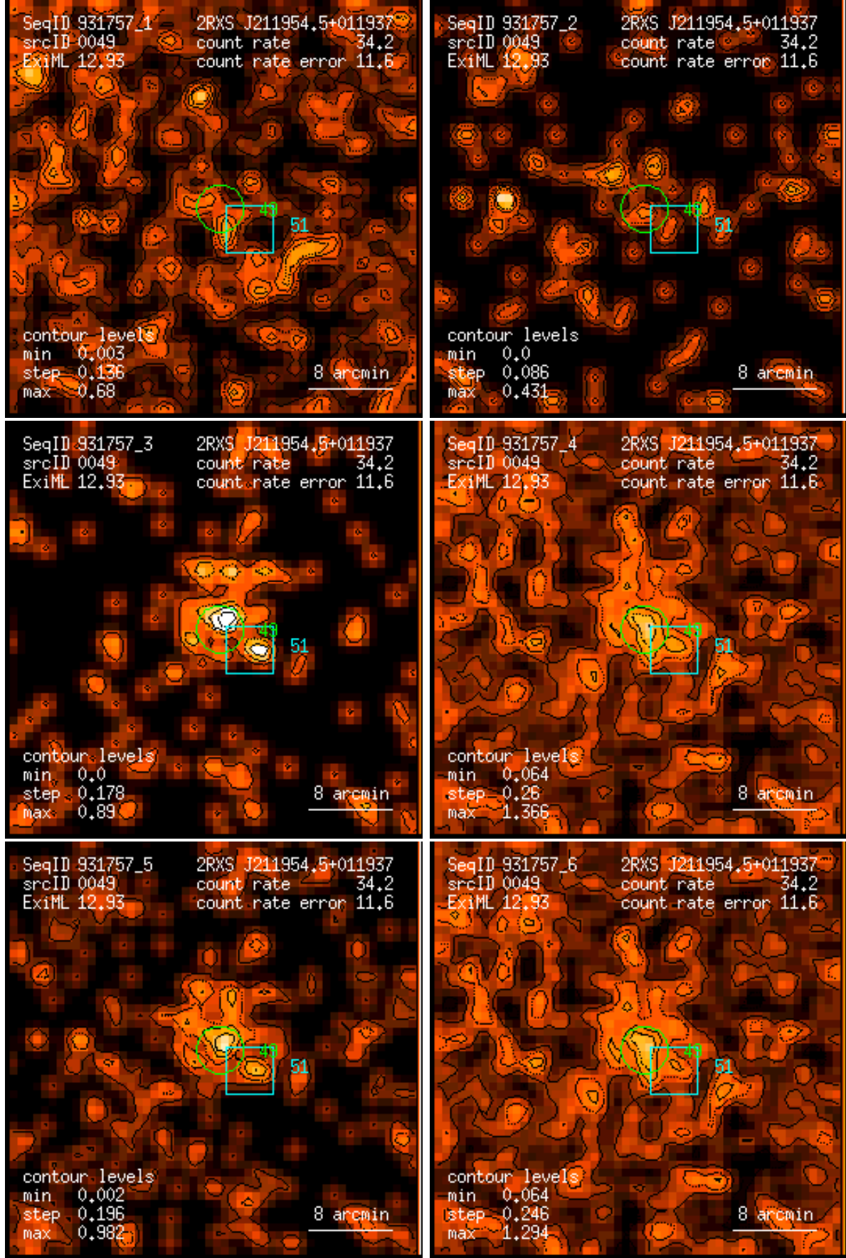
Figure 49: RASS 931757: detection 0049: band rate images, Gaussian filter: (1) PSPC channels 11 – 41, (2) 52 – 90, (3) 91 – 201, (4) 11 – 235, (5) 52 – 201, (6) 11 – 201. Broad band rates in counts/ks. Band rate contour levels in counts/ks/arcmin 2 .
