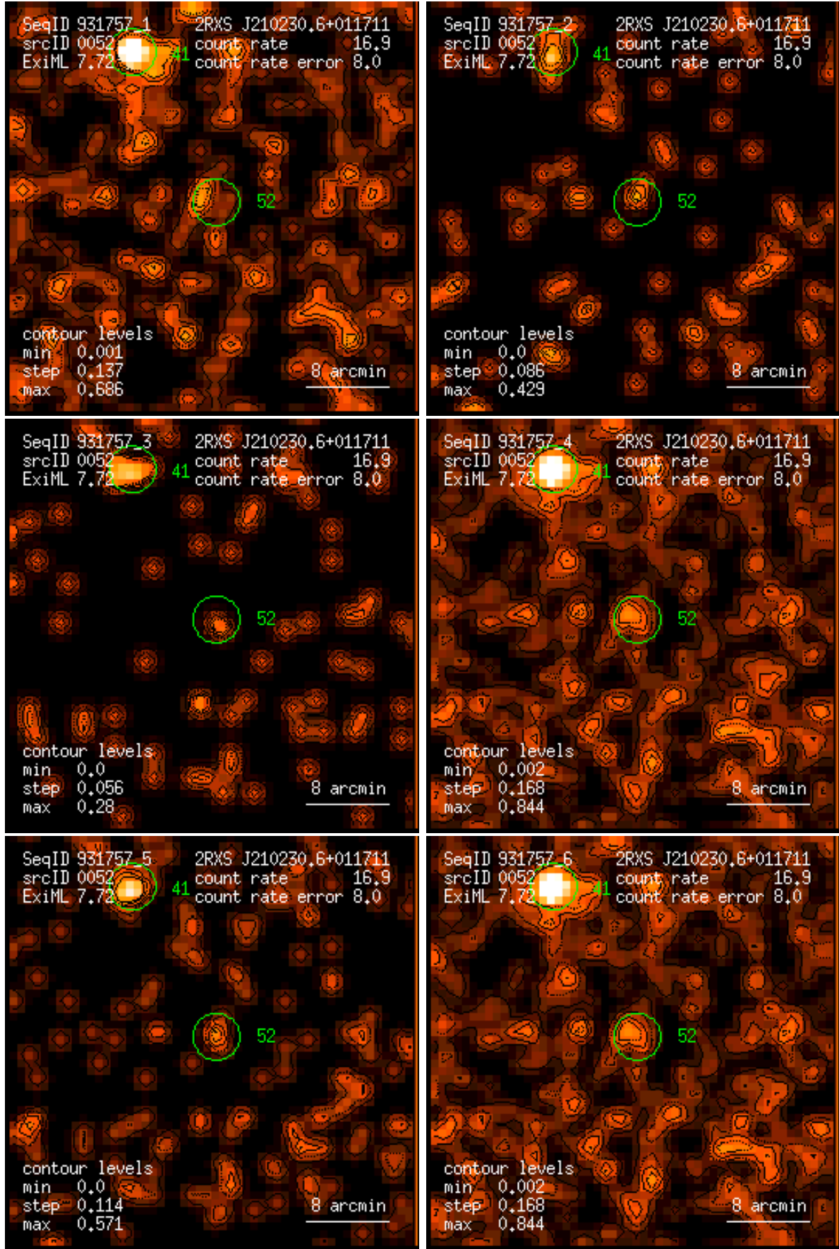
Figure 52: RASS 931757: detection 0052: band rate images, Gaussian filter: (1) PSPC channels 11 – 41, (2) 52 – 90, (3) 91 – 201, (4) 11 – 235, (5) 52 – 201, (6) 11 – 201. Broad band rates in counts/ks. Band rate contour levels in counts/ks/arcmin 2 .
