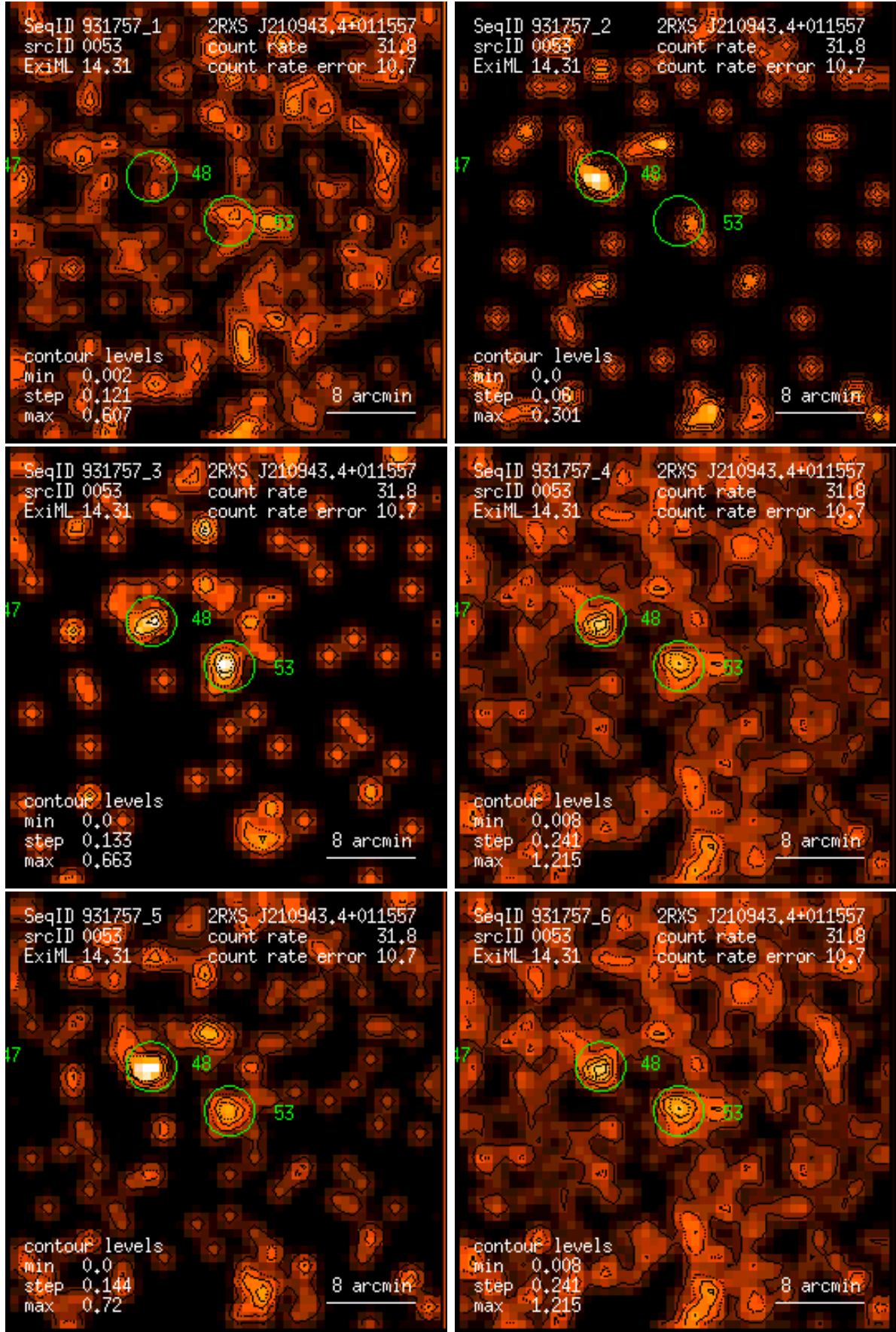
Figure 53: RASS 931757: detection 0053: band rate images, Gaussian filter: (1) PSPC channels 11 – 41, (2) 52 – 90, (3) 91 – 201, (4) 11 – 235, (5) 52 – 201, (6) 11 – 201. Broad band rates in counts/ks. Band rate contour levels in counts/ks/arcmin 2 .
