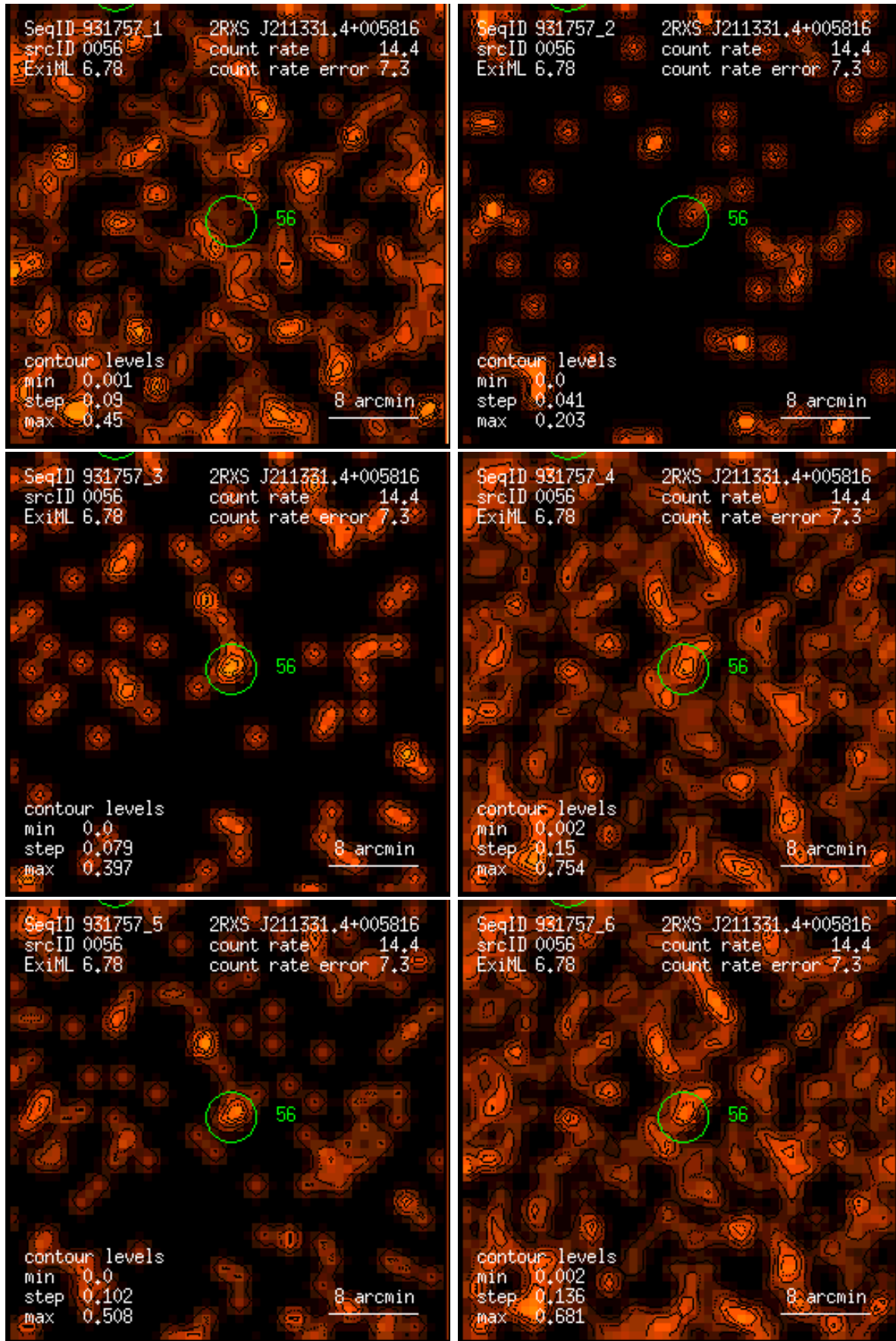
Figure 56: RASS 931757: detection 0056: band rate images, Gaussian filter: (1) PSPC channels 11 – 41, (2) 52 – 90, (3) 91 – 201, (4) 11 – 235, (5) 52 – 201, (6) 11 – 201. Broad band rates in counts/ks. Band rate contour levels in counts/ks/arcmin 2 .
