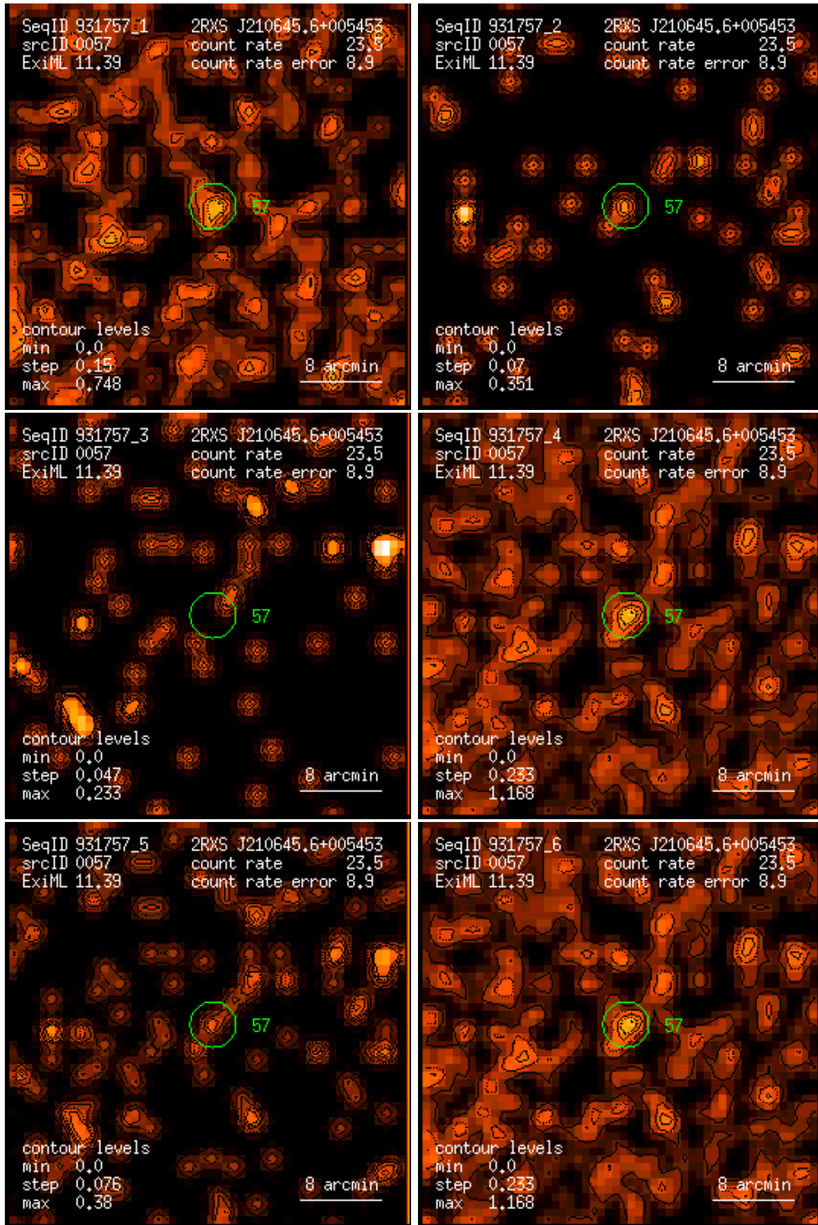
Figure 57: RASS 931757: detection 0057: band rate images, Gaussian filter: (1) PSPC channels 11 – 41, (2) 52 – 90, (3) 91 – 201, (4) 11 – 235, (5) 52 – 201, (6) 11 – 201. Broad band rates in counts/ks. Band rate contour levels in counts/ks/arcmin 2 .
