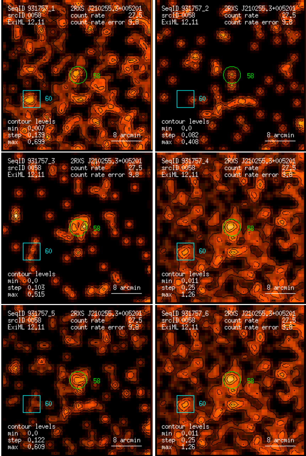
Figure 58: RASS 931757: detection 0058: band rate images, Gaussian filter: (1) PSPC channels 11 – 41, (2) 52 – 90, (3) 91 – 201, (4) 11 – 235, (5) 52 – 201, (6) 11 – 201. Broad band rates in counts/ks. Band rate contour levels in counts/ks/arcmin 2 .
