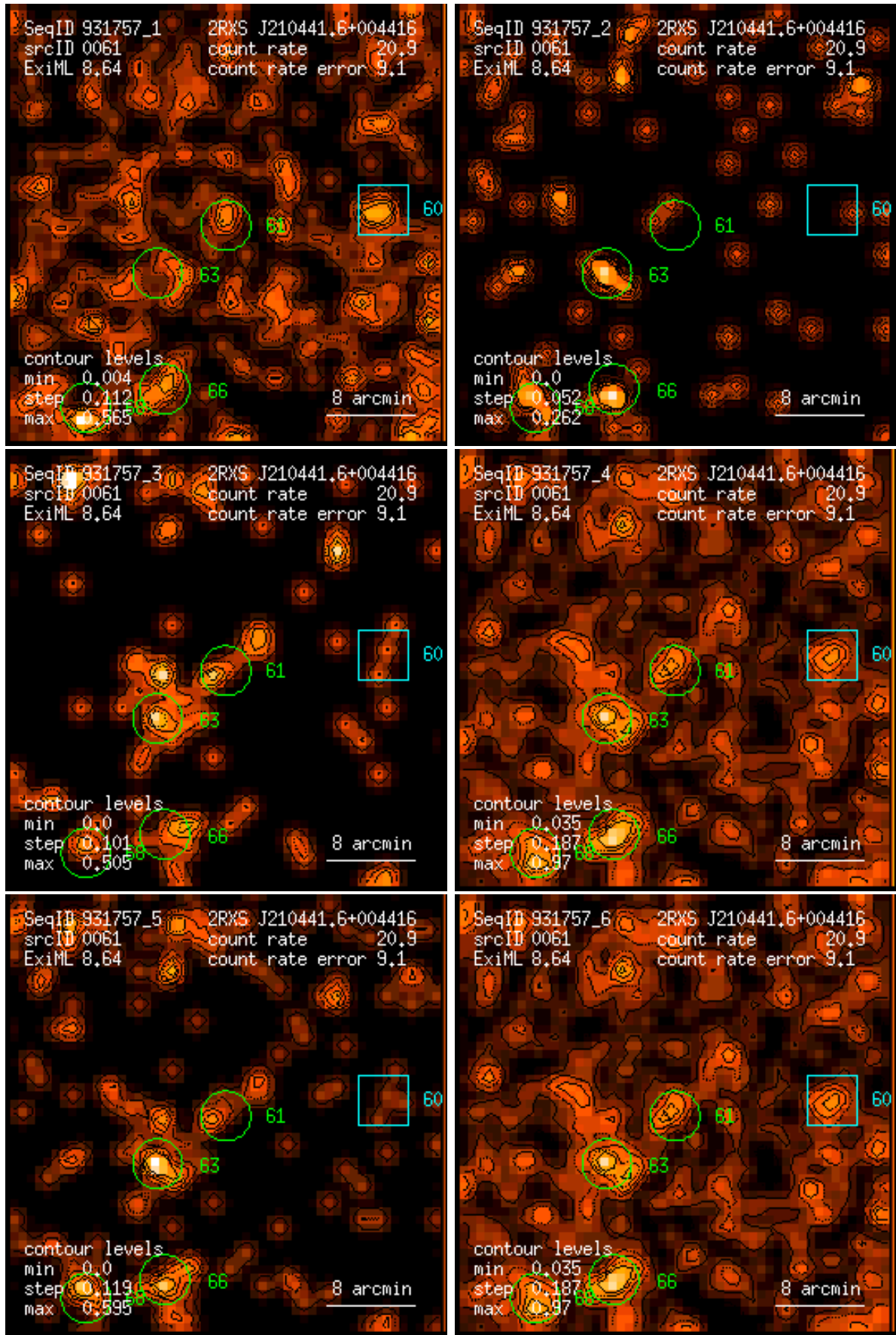
Figure 61: RASS 931757: detection 0061: band rate images, Gaussian filter: (1) PSPC channels 11 – 41, (2) 52 – 90, (3) 91 – 201, (4) 11 – 235, (5) 52 – 201, (6) 11 – 201. Broad band rates in counts/ks. Band rate contour levels in counts/ks/arcmin 2 .
