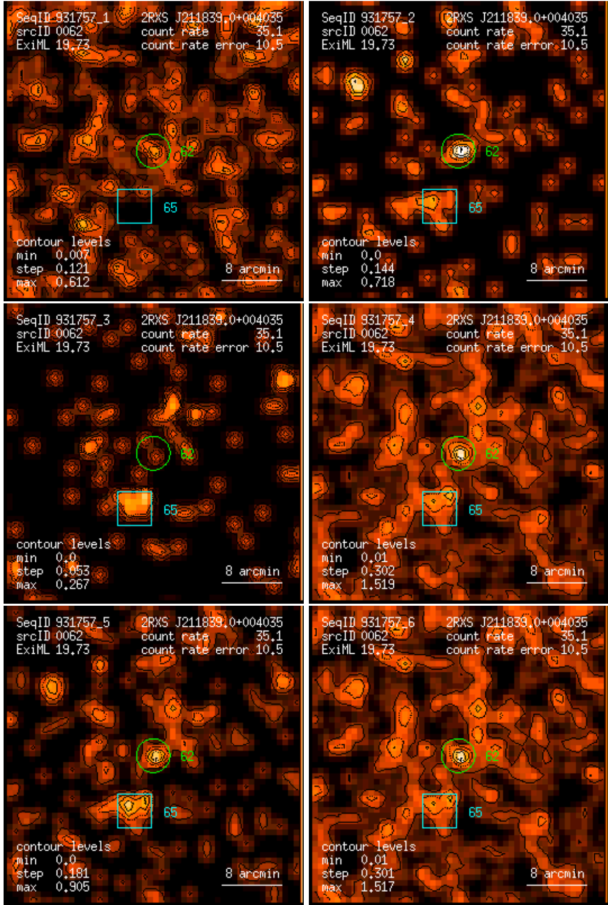
Figure 62: RASS 931757: detection 0062: band rate images, Gaussian filter: (1) PSPC channels 11 – 41, (2) 52 – 90, (3) 91 – 201, (4) 11 – 235, (5) 52 – 201, (6) 11 – 201. Broad band rates in counts/ks. Band rate contour levels in counts/ks/arcmin 2 .
