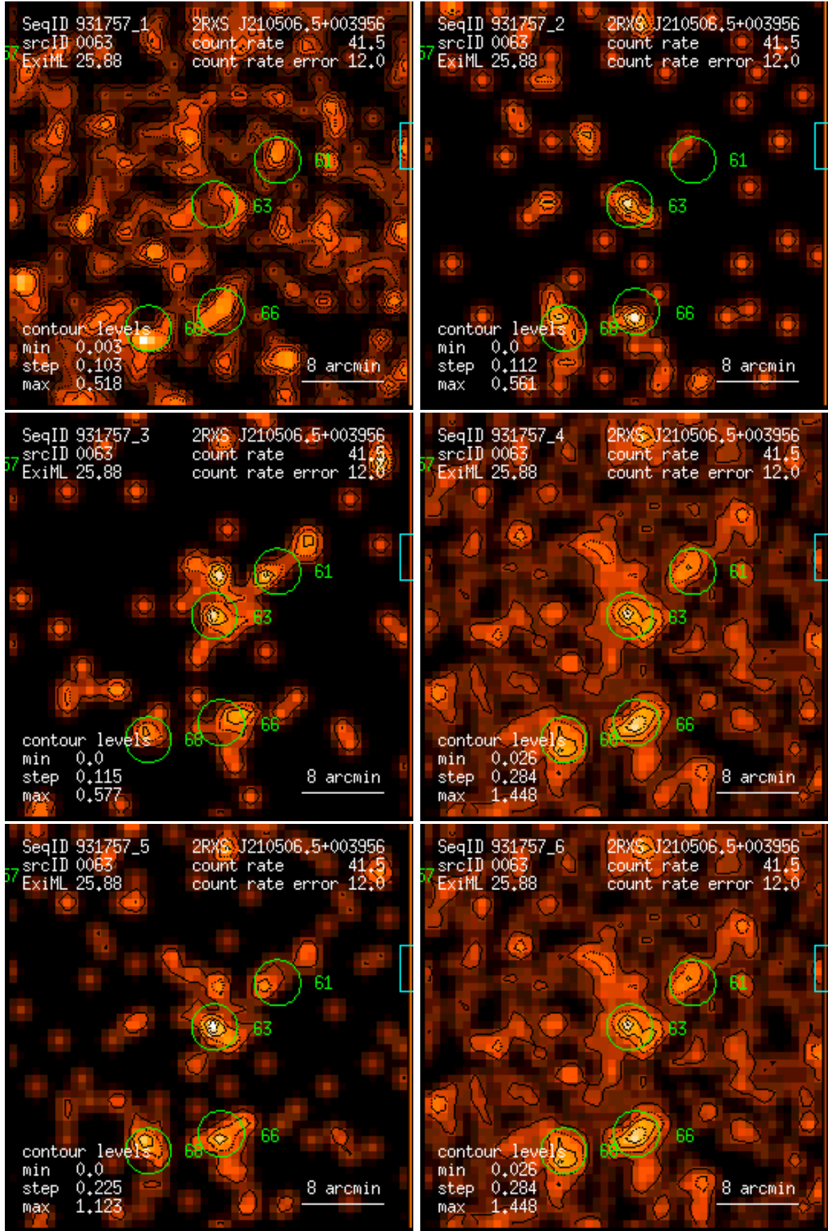
Figure 63: RASS 931757: detection 0063: band rate images, Gaussian filter: (1) PSPC channels 11 – 41, (2) 52 – 90, (3) 91 – 201, (4) 11 – 235, (5) 52 – 201, (6) 11 – 201. Broad band rates in counts/ks. Band rate contour levels in counts/ks/arcmin 2 .
