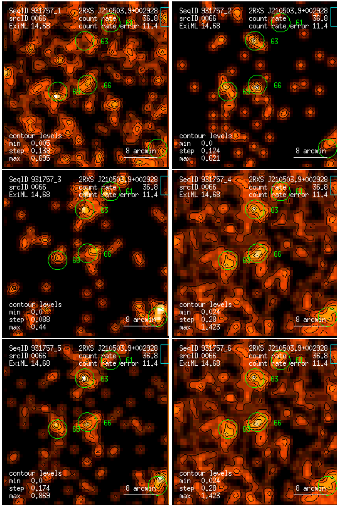
Figure 66: RASS 931757: detection 0066: band rate images, Gaussian filter: (1) PSPC channels 11 – 41, (2) 52 – 90, (3) 91 – 201, (4) 11 – 235, (5) 52 – 201, (6) 11 – 201. Broad band rates in counts/ks. Band rate contour levels in counts/ks/arcmin 2 .
