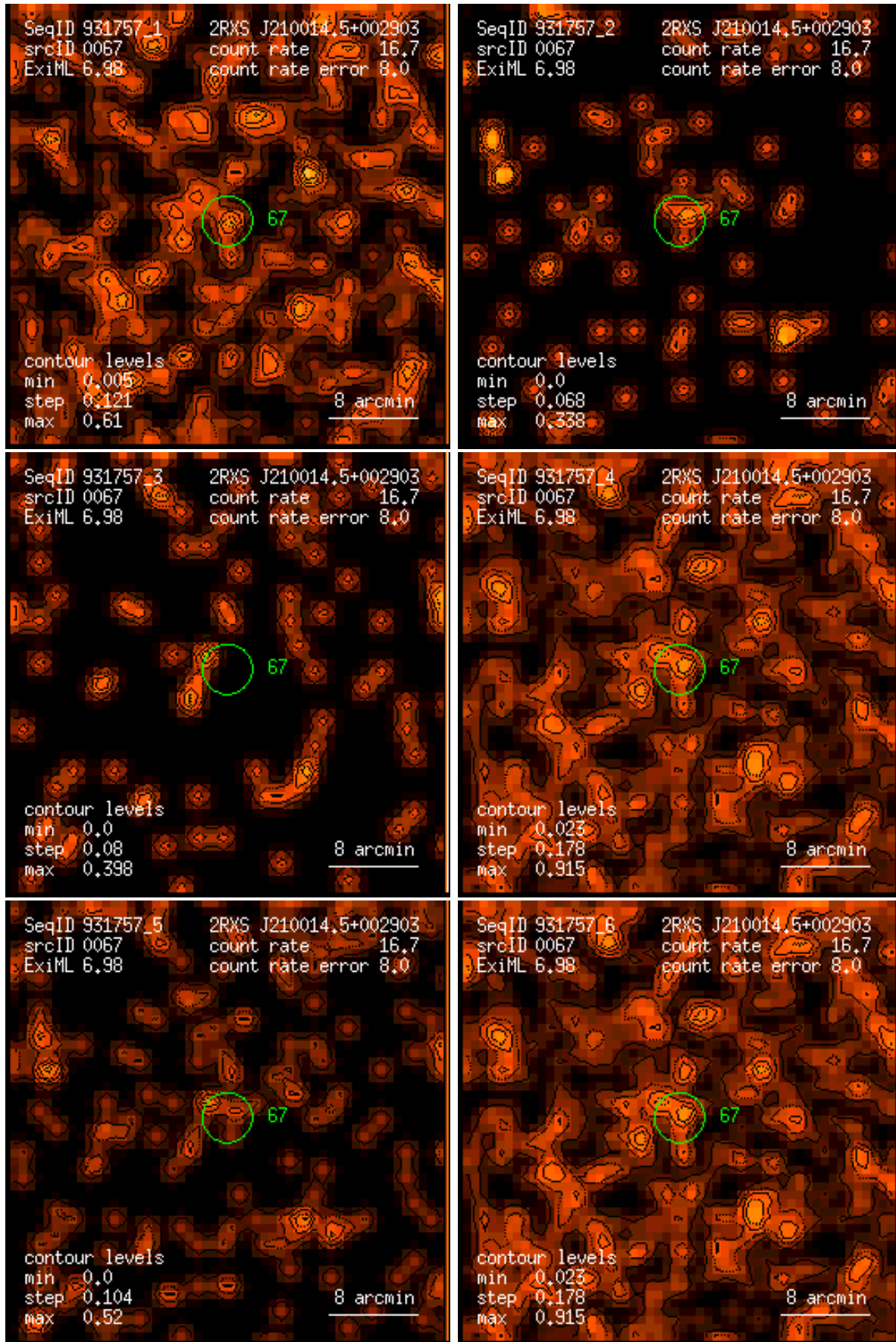
Figure 67: RASS 931757: detection 0067: band rate images, Gaussian filter: (1) PSPC channels 11 – 41, (2) 52 – 90, (3) 91 – 201, (4) 11 – 235, (5) 52 – 201, (6) 11 – 201. Broad band rates in counts/ks. Band rate contour levels in counts/ks/arcmin 2 .
