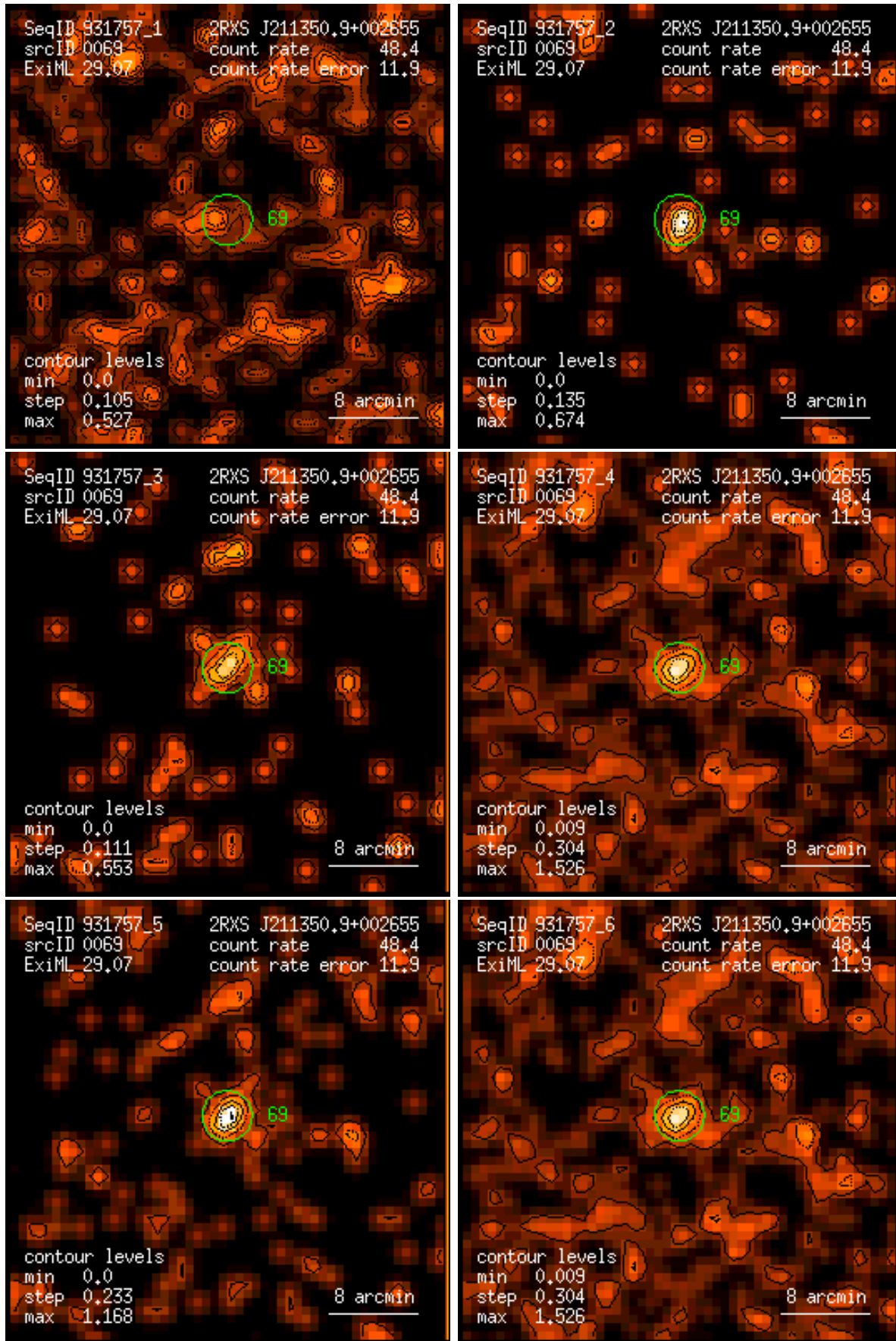
Figure 69: RASS 931757: detection 0069: band rate images, Gaussian filter: (1) PSPC channels 11 – 41, (2) 52 – 90, (3) 91 – 201, (4) 11 – 235, (5) 52 – 201, (6) 11 – 201. Broad band rates in counts/ks. Band rate contour levels in counts/ks/arcmin 2 .
