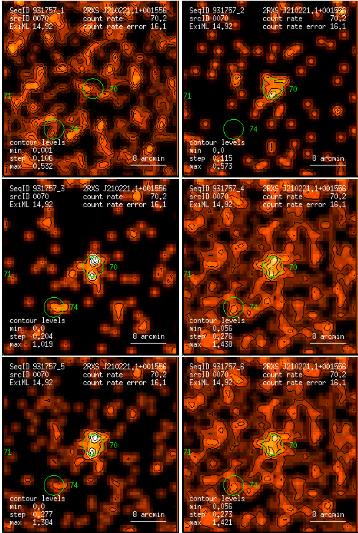
Figure 70: RASS 931757: detection 0070: band rate images, Gaussian filter: (1) PSPC channels 11 – 41, (2) 52 – 90, (3) 91 – 201, (4) 11 – 235, (5) 52 – 201, (6) 11 – 201. Broad band rates in counts/ks. Band rate contour levels in counts/ks/arcmin 2 .
