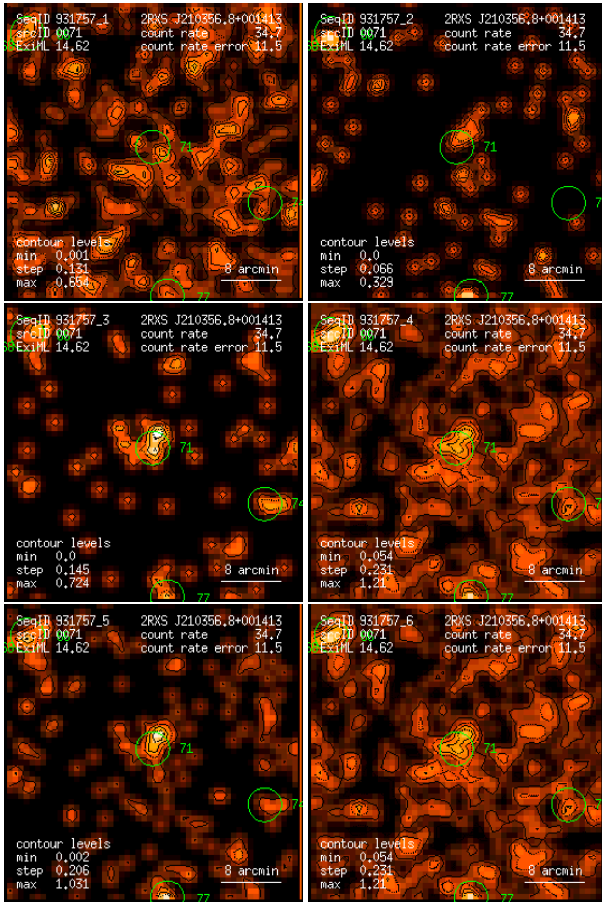
Figure 71: RASS 931757: detection 0071: band rate images, Gaussian filter: (1) PSPC channels 11 – 41, (2) 52 – 90, (3) 91 – 201, (4) 11 – 235, (5) 52 – 201, (6) 11 – 201. Broad band rates in counts/ks. Band rate contour levels in counts/ks/arcmin 2 .
