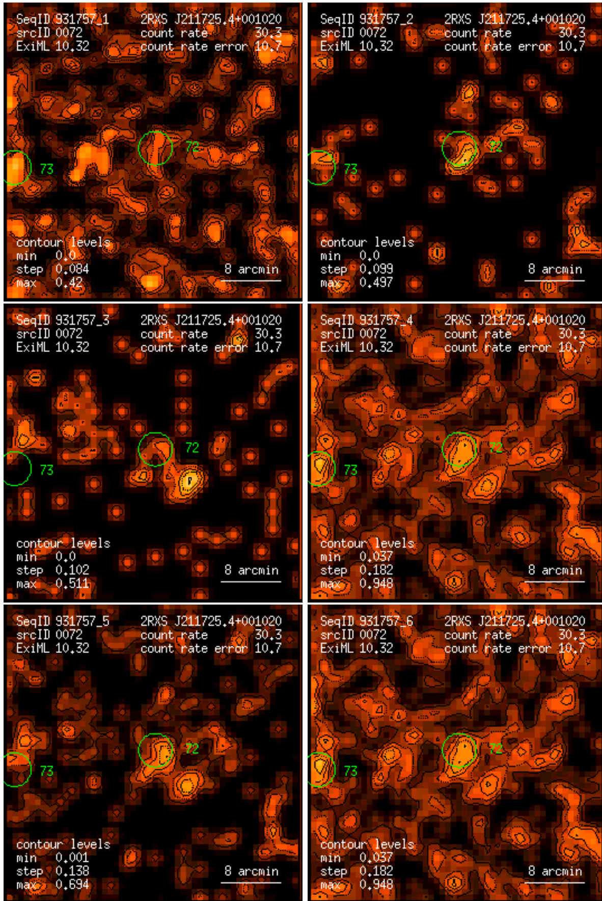
Figure 72: RASS 931757: detection 0072: band rate images, Gaussian filter: (1) PSPC channels 11 – 41, (2) 52 – 90, (3) 91 – 201, (4) 11 – 235, (5) 52 – 201, (6) 11 – 201. Broad band rates in counts/ks. Band rate contour levels in counts/ks/arcmin 2 .
