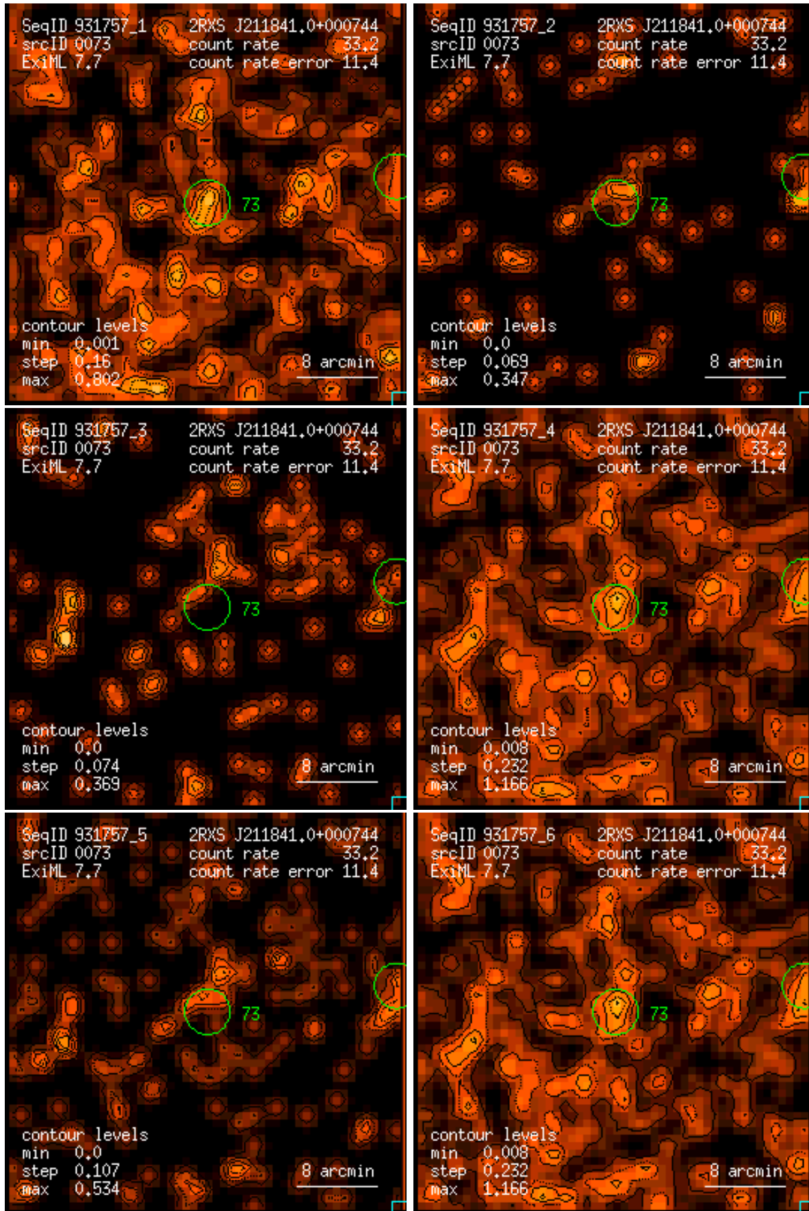
Figure 73: RASS 931757: detection 0073: band rate images, Gaussian filter: (1) PSPC channels 11 – 41, (2) 52 – 90, (3) 91 – 201, (4) 11 – 235, (5) 52 – 201, (6) 11 – 201. Broad band rates in counts/ks. Band rate contour levels in counts/ks/arcmin 2 .
