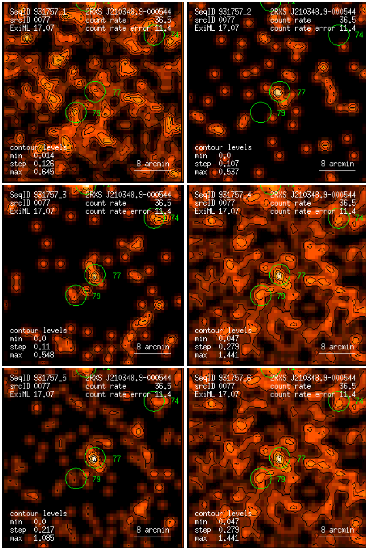
Figure 77: RASS 931757: detection 0077: band rate images, Gaussian filter: (1) PSPC channels 11 – 41, (2) 52 – 90, (3) 91 – 201, (4) 11 – 235, (5) 52 – 201, (6) 11 – 201. Broad band rates in counts/ks. Band rate contour levels in counts/ks/arcmin 2 .
