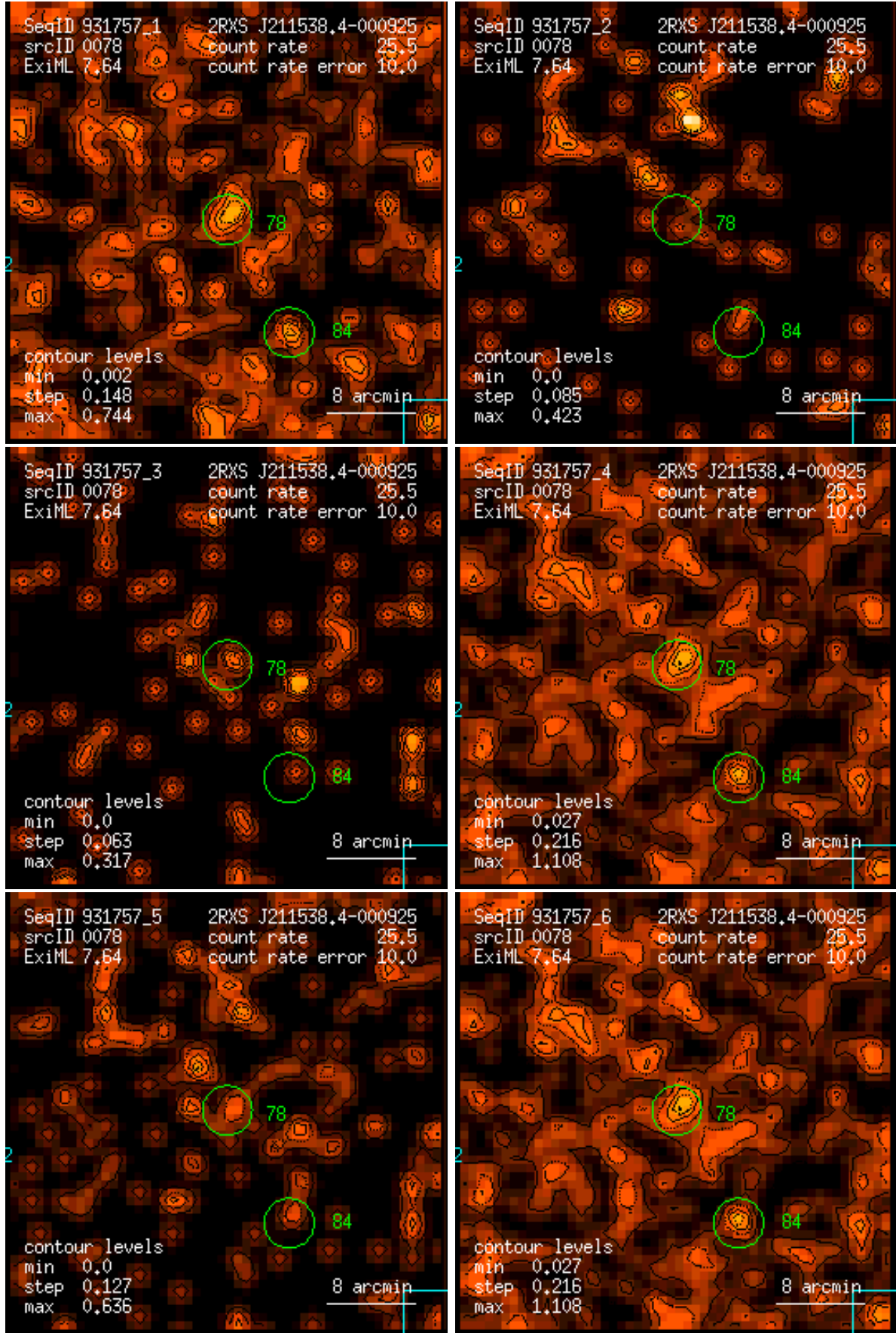
Figure 78: RASS 931757: detection 0078: band rate images, Gaussian filter: (1) PSPC channels 11 – 41, (2) 52 – 90, (3) 91 – 201, (4) 11 – 235, (5) 52 – 201, (6) 11 – 201. Broad band rates in counts/ks. Band rate contour levels in counts/ks/arcmin 2 .
