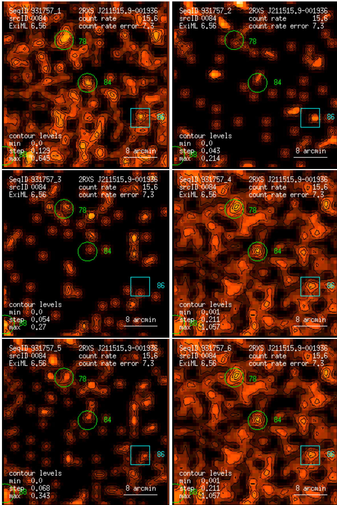
Figure 84: RASS 931757: detection 0084: band rate images, Gaussian filter: (1) PSPC channels 11 – 41, (2) 52 – 90, (3) 91 – 201, (4) 11 – 235, (5) 52 – 201, (6) 11 – 201. Broad band rates in counts/ks. Band rate contour levels in counts/ks/arcmin 2 .
