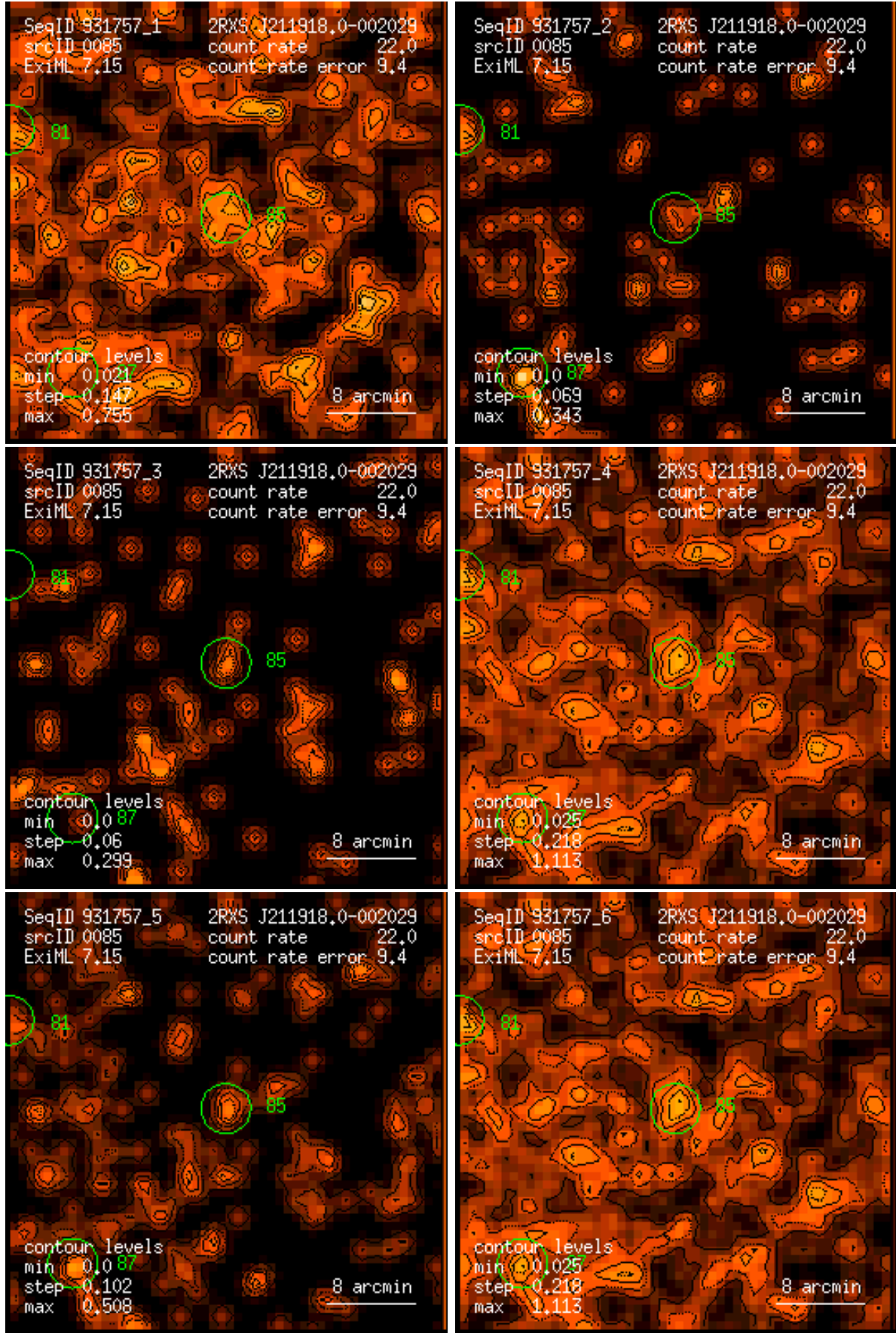
Figure 85: RASS 931757: detection 0085: band rate images, Gaussian filter: (1) PSPP channels 11 – 41, (2) 52 – 90, (3) 91 – 201, (4) 11 – 235, (5) 52 – 201, (6) 11 – 201. Broad band rates in counts/ks. Band rate contour levels in counts/ks/arcmin 2 .
