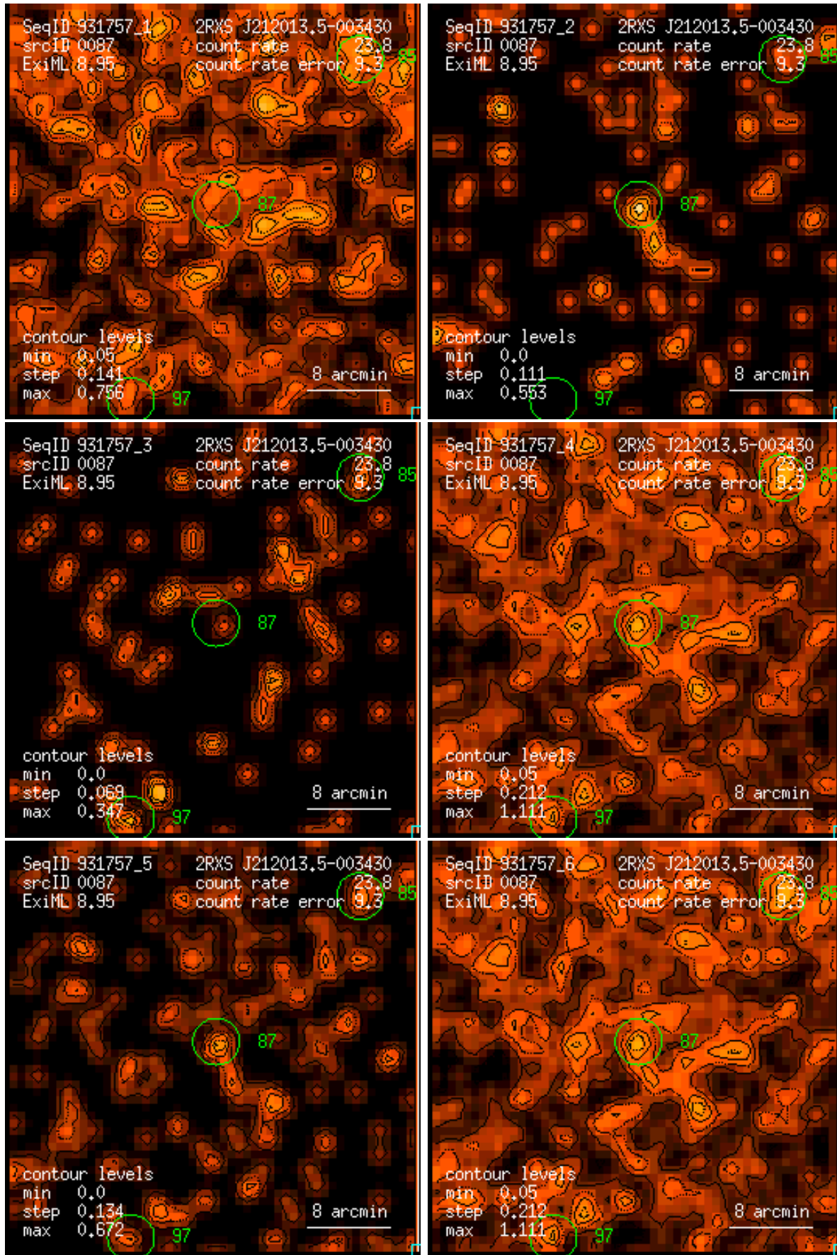
Figure 87: RASS 931757: detection 0087: band rate images, Gaussian filter: (1) PSPC channels 11 – 41, (2) 52 – 90, (3) 91 – 201, (4) 11 – 235, (5) 52 – 201, (6) 11 – 201. Broad band rates in counts/ks. Band rate contour levels in counts/ks/arcmin 2 .
