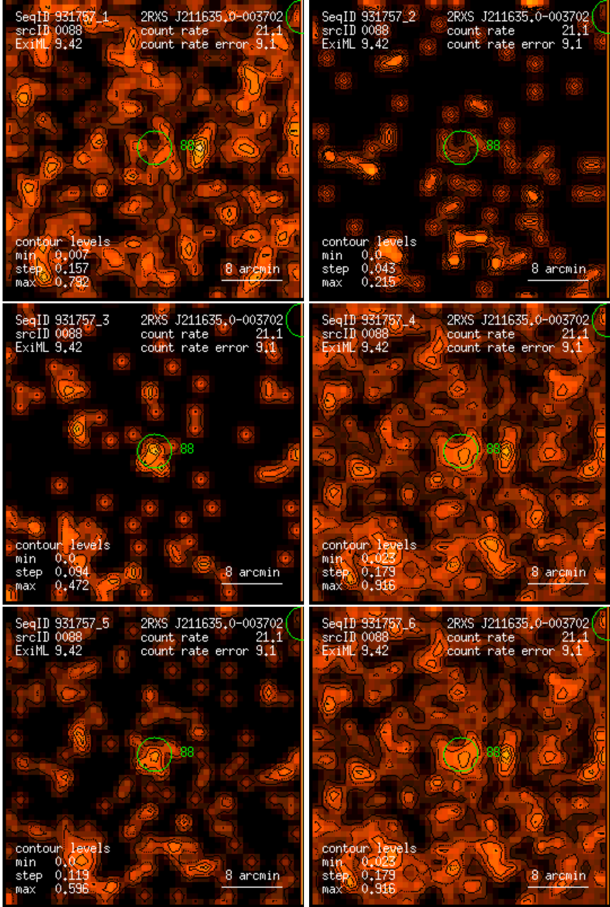
Figure 88: RASS 931757: detection 0088: band rate images, Gaussian filter: (1) PSPC channels 11 – 41, (2) 52 – 90, (3) 91 – 201, (4) 11 – 235, (5) 52 – 201, (6) 11 – 201. Broad band rates in counts/ks. Band rate contour levels in counts/ks/arcmin 2 .
