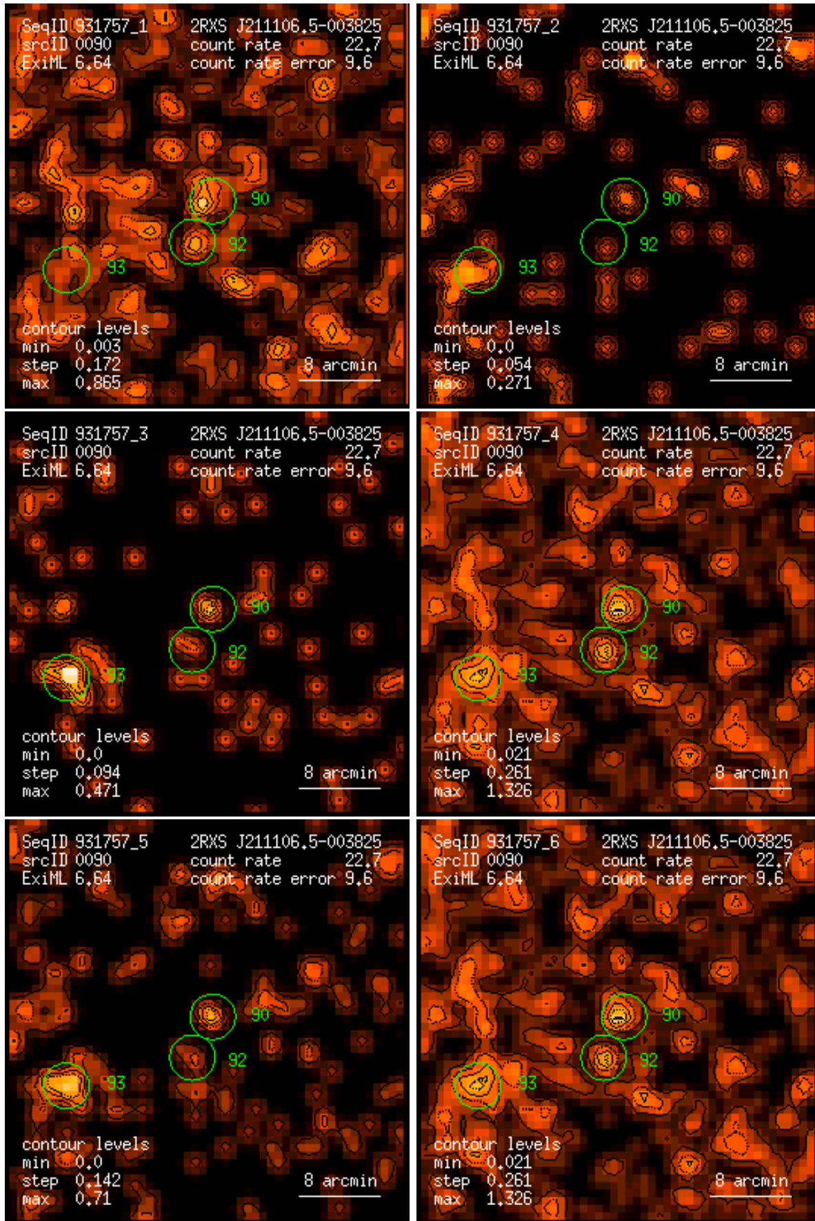
Figure 90: RASS 931757: detection 0090: band rate images, Gaussian filter: (1) PSPC channels 11 – 41, (2) 52 – 90, (3) 91 – 201, (4) 11 – 235, (5) 52 – 201, (6) 11 – 201. Broad band rates in counts/ks. Band rate contour levels in counts/ks/arcmin 2 .
