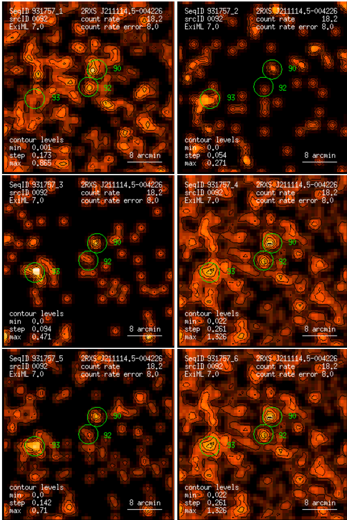
Figure 92: RASS 931757: detection 0092: band rate images, Gaussian filter: (1) PSPC channels 11 – 41, (2) 52 – 90, (3) 91 – 201, (4) 11 – 235, (5) 52 – 201, (6) 11 – 201. Broad band rates in counts/ks. Band rate contour levels in counts/ks/arcmin 2 .
