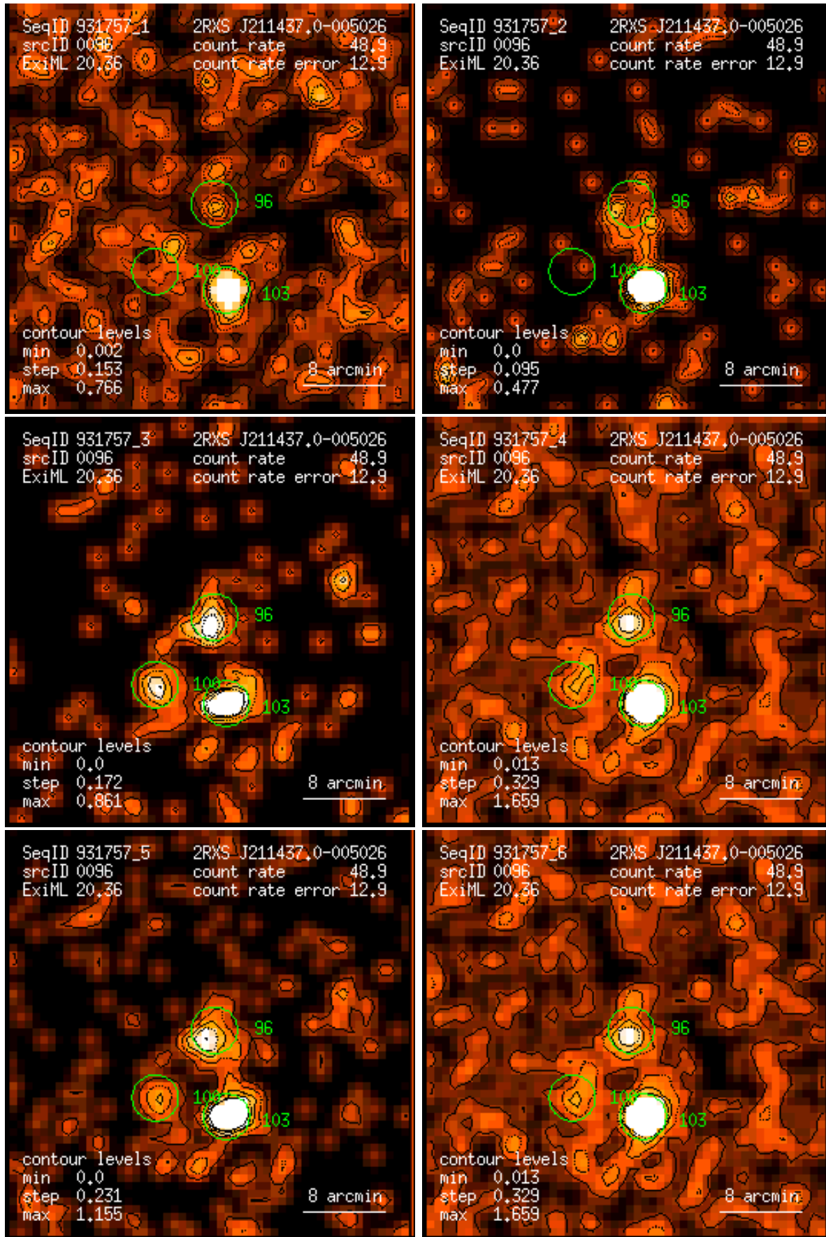
Figure 96: RASS 931757: detection 0096: band rate images, Gaussian filter: (1) PSPC channels 11 – 41, (2) 52 – 90, (3) 91 – 201, (4) 11 – 235, (5) 52 – 201, (6) 11 – 201. Broad band rates in counts/ks. Band rate contour levels in counts/ks/arcmin 2 .
