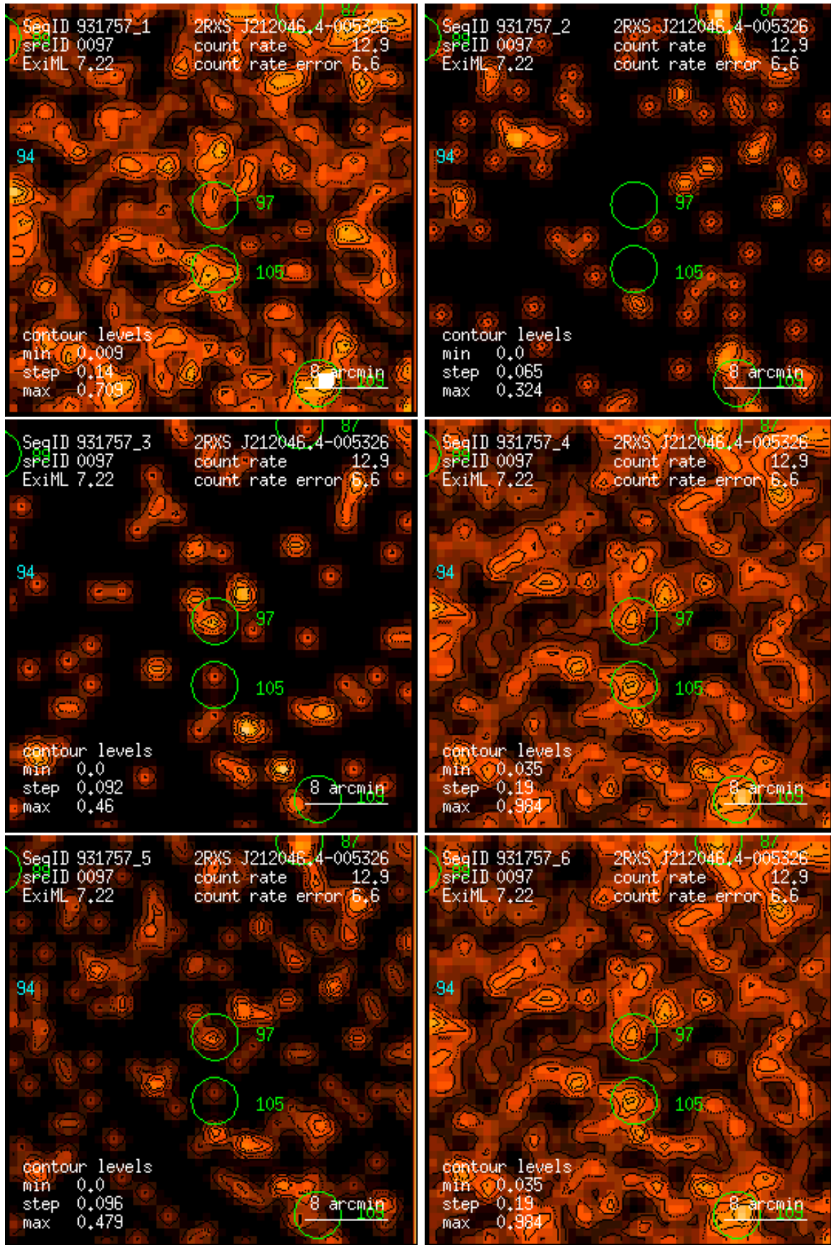
Figure 97: RASS 931757: detection 0097: band rate images, Gaussian filter: (1) PSPC channels 11 – 41, (2) 52 – 90, (3) 91 – 201, (4) 11 – 235, (5) 52 – 201, (6) 11 – 201. Broad band rates in counts/ks. Band rate contour levels in counts/ks/arcmin 2 .
