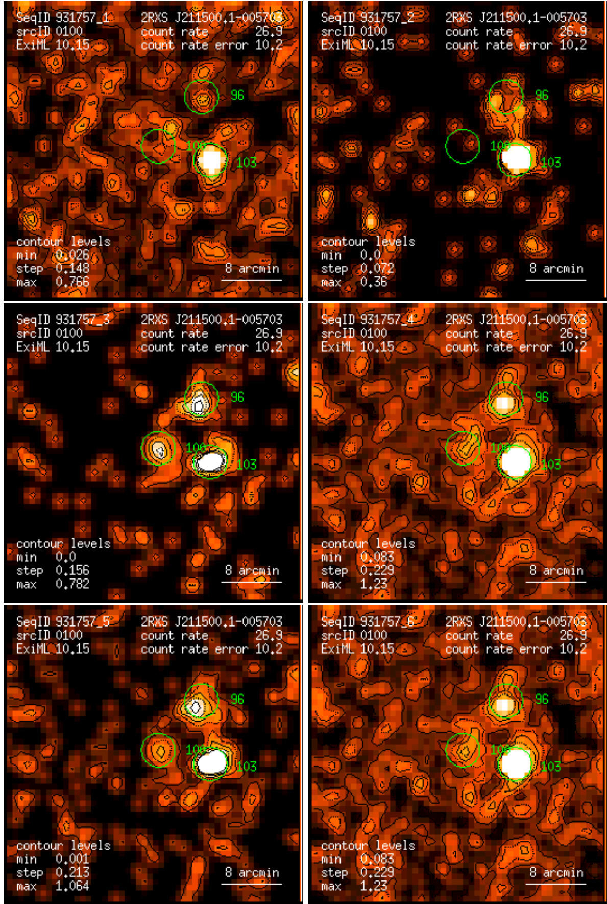
Figure 100: RASS 931757: detection 0100: band rate images, Gaussian filter: (1) PSPC channels 11 – 41, (2) 52 – 90, (3) 91 – 201, (4) 11 – 235, (5) 52 – 201, (6) 11 – 201. Broad band rates in counts/ks. Band rate contour levels in counts/ks/arcmin 2 .
