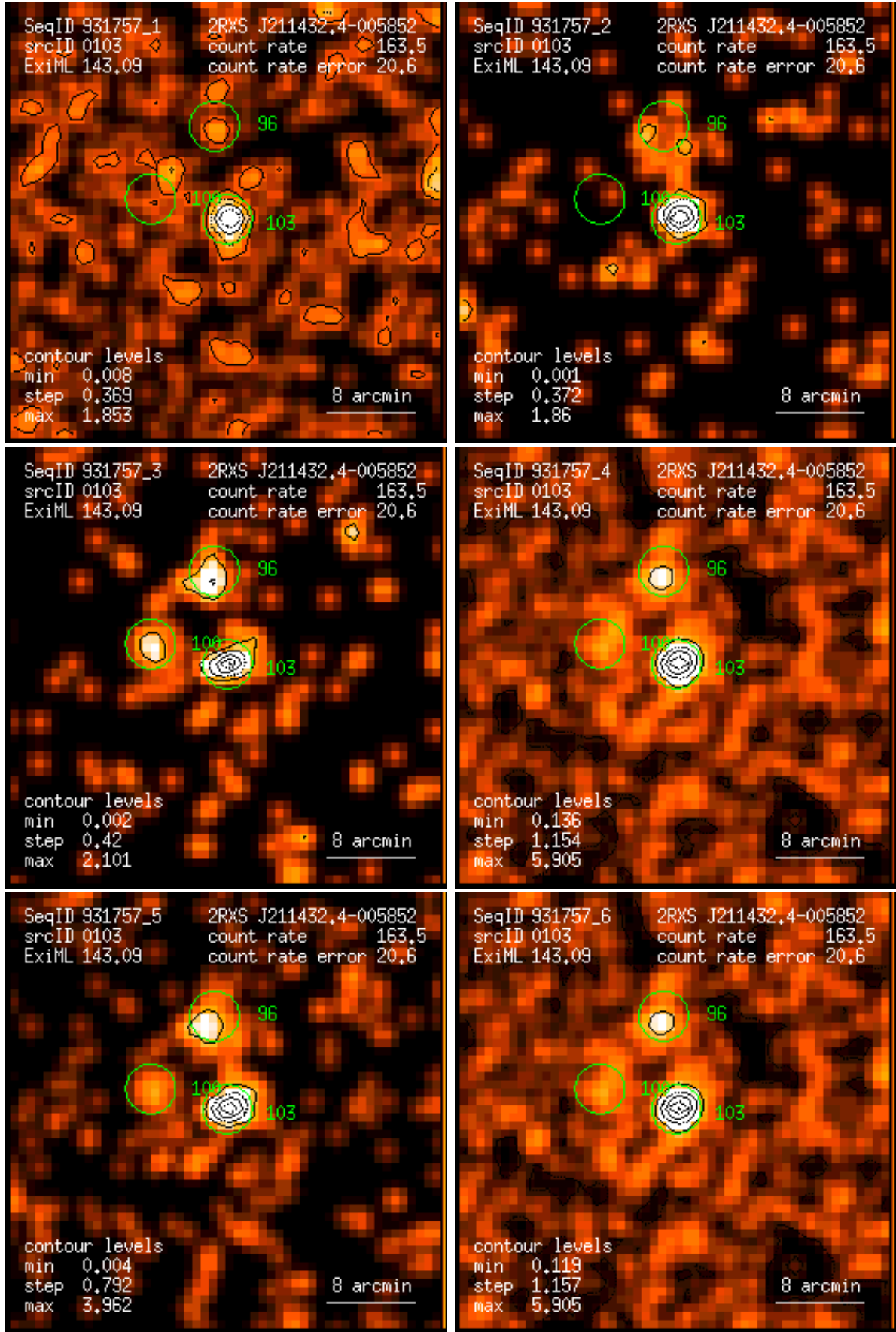
Figure 103: RASS 931757: detection 0103: band rate images, Gaussian filter: (1) PSPC channels 11 – 41, (2) 52 – 90, (3) 91 – 201, (4) 11 – 235, (5) 52 – 201, (6) 11 – 201. Broad band rates in counts/ks. Band rate contour levels in counts/ks/arcmin 2 .
