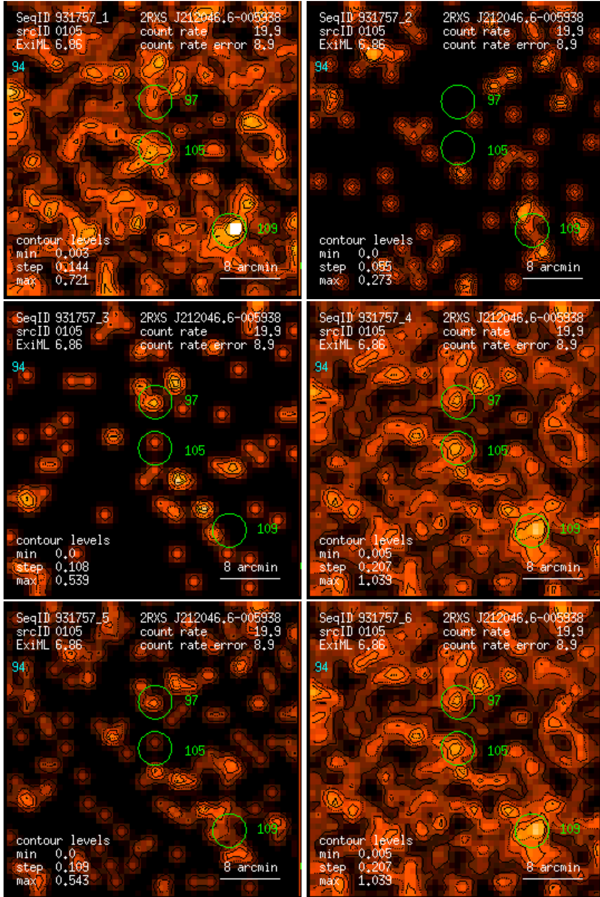
Figure 105: RASS 931757: detection 0105: band rate images, Gaussian filter: (1) PSPC channels 11 – 41, (2) 52 – 90, (3) 91 – 201, (4) 11 – 235, (5) 52 – 201, (6) 11 – 201. Broad band rates in counts/ks. Band rate contour levels in counts/ks/arcmin 2 .
