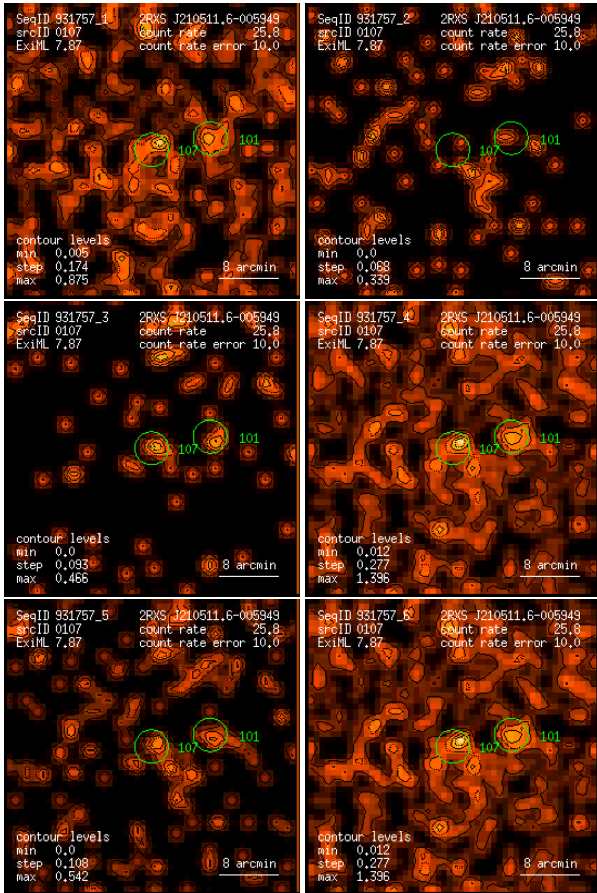
Figure 107: RASS 931757: detection 0107: band rate images, Gaussian filter: (1) PSPC channels 11 – 41, (2) 52 – 90, (3) 91 – 201, (4) 11 – 235, (5) 52 – 201, (6) 11 – 201. Broad band rates in counts/ks. Band rate contour levels in counts/ks/arcmin 2 .
