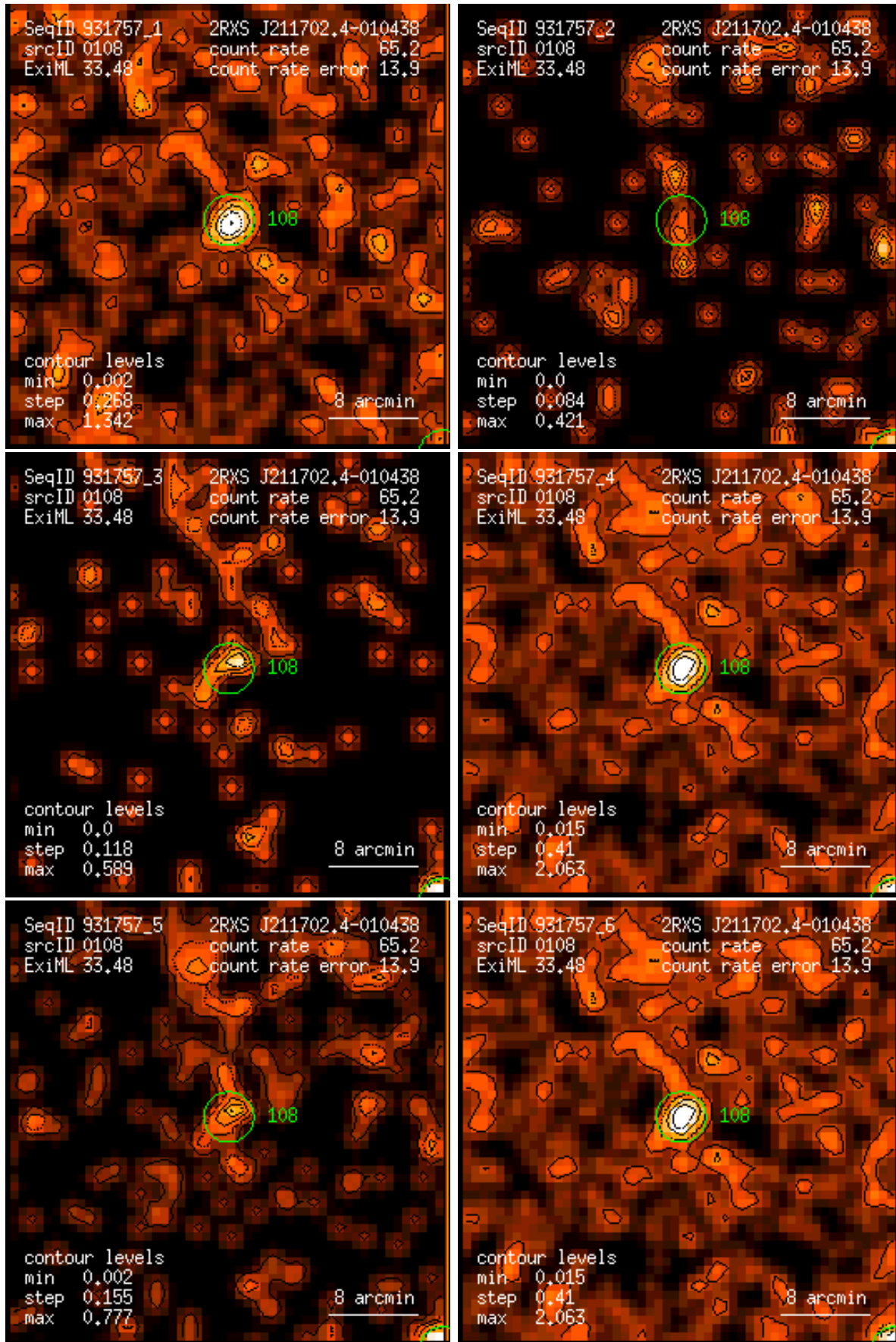
Figure 108: RASS 931757: detection 0108: band rate images, Gaussian filter: (1) PSPC channels 11 – 41, (2) 52 – 90, (3) 91 – 201, (4) 11 – 235, (5) 52 – 201, (6) 11 – 201. Broad band rates in counts/ks. Band rate contour levels in counts/ks/arcmin 2 .
