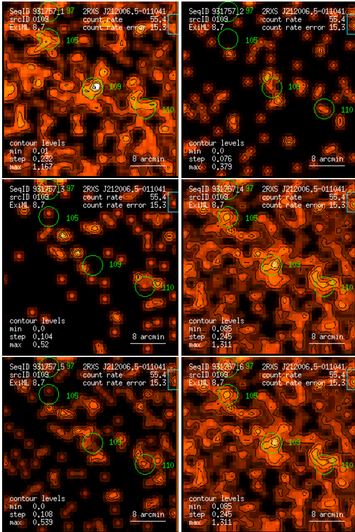
Figure 109: RASS 931757: detection 0109: band rate images, Gaussian filter: (1) PSPC channels 11 – 41, (2) 52 – 90, (3) 91 – 201, (4) 11 – 235, (5) 52 – 201, (6) 11 – 201. Broad band rates in counts/ks. Band rate contour levels in counts/ks/arcmin 2 .
