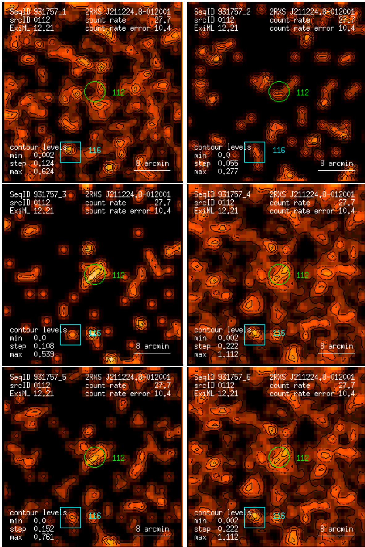
Figure 112: RASS 931757: detection 0112: band rate images, Gaussian filter: (1) PSPC channels 11 – 41, (2) 52 – 90, (3) 91 – 201, (4) 11 – 235, (5) 52 – 201, (6) 11 – 201. Broad band rates in counts/ks. Band rate contour levels in counts/ks/arcmin 2 .
