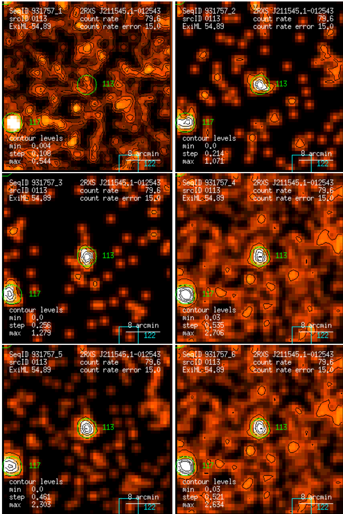
Figure 113: RASS 931757: detection 0113: band rate images, Gaussian filter: (1) PSPC channels 11 – 41, (2) 52 – 90, (3) 91 – 201, (4) 11 – 235, (5) 52 – 201, (6) 11 – 201. Broad band rates in counts/ks. Band rate contour levels in counts/ks/arcmin 2 .
