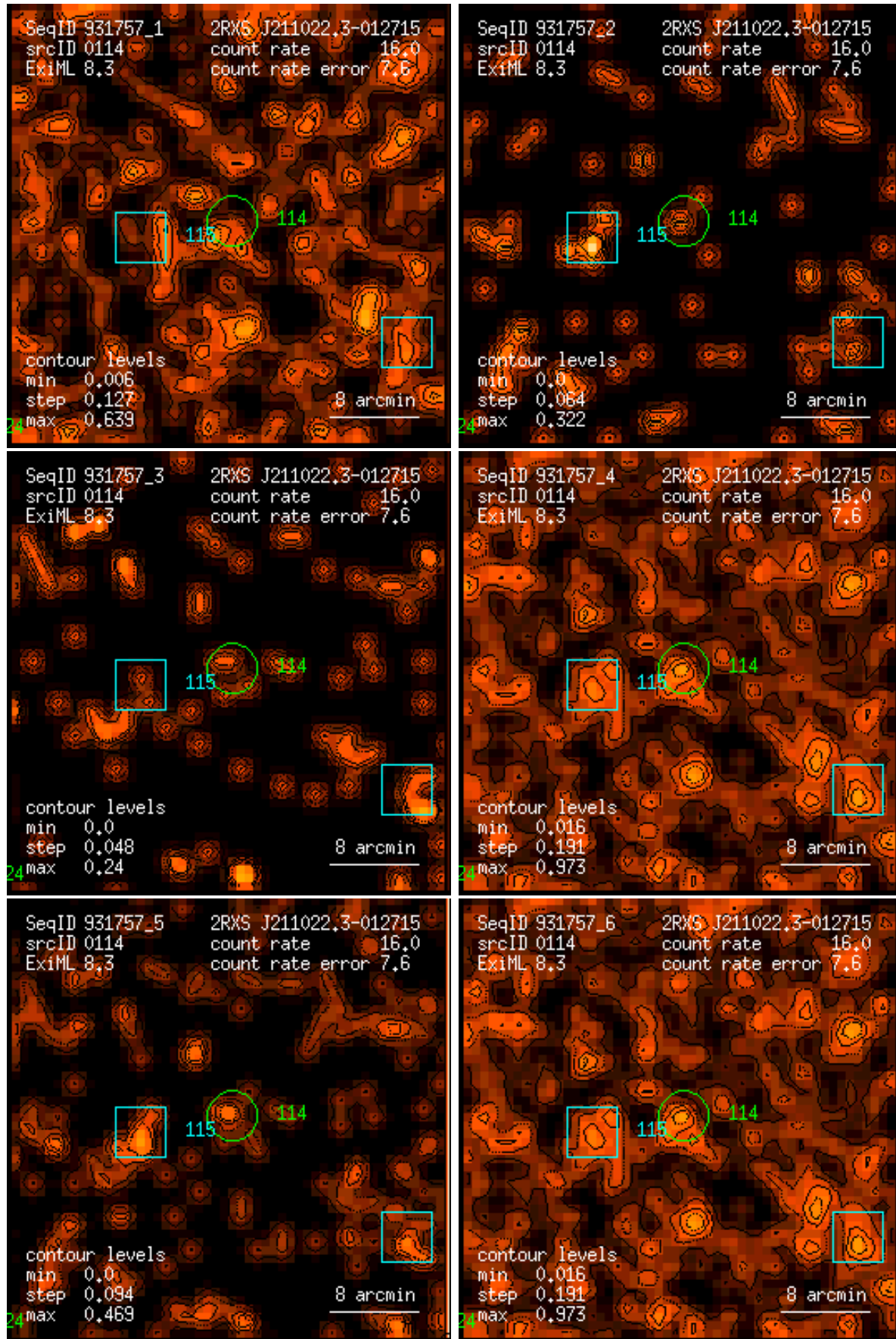
Figure 114: RASS 931757: detection 0114: band rate images, Gaussian filter: (1) PSPC channels 11 – 41, (2) 52 – 90, (3) 91 – 201, (4) 11 – 235, (5) 52 – 201, (6) 11 – 201. Broad band rates in counts/ks. Band rate contour levels in counts/ks/arcmin 2 .
