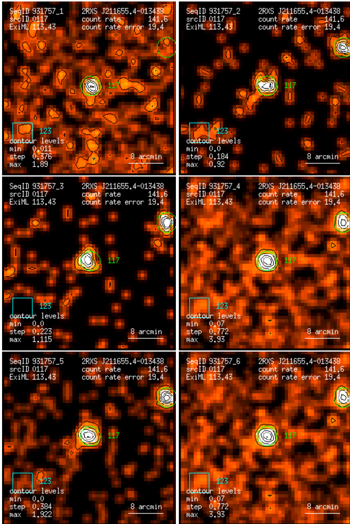
Figure 117: RASS 931757: detection 0117: band rate images, Gaussian filter: (1) PSPC channels 11 – 41, (2) 52 – 90, (3) 91 – 201, (4) 11 – 235, (5) 52 – 201, (6) 11 – 201. Broad band rates in counts/ks. Band rate contour levels in counts/ks/arcmin 2 .
